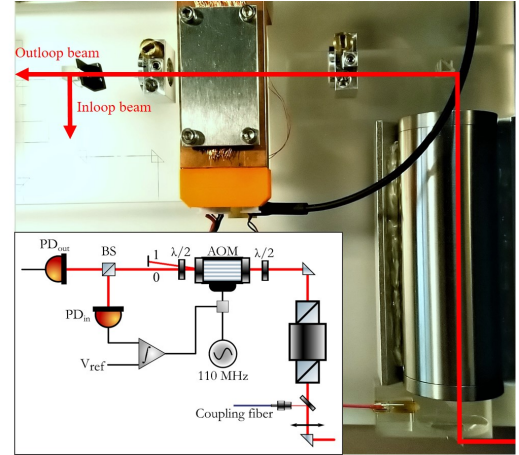
Fig. 1: Miniature optical bench for the optical power stabilization. AOM: Acousto-optic modulator; BS: Beamsplitter; PD: Photodetectors.
