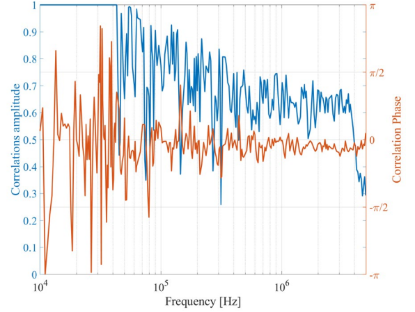
Fig. 5: Amplitude and phase of intensity noise correlation between the two polarizations emitted by the VECSEL.
