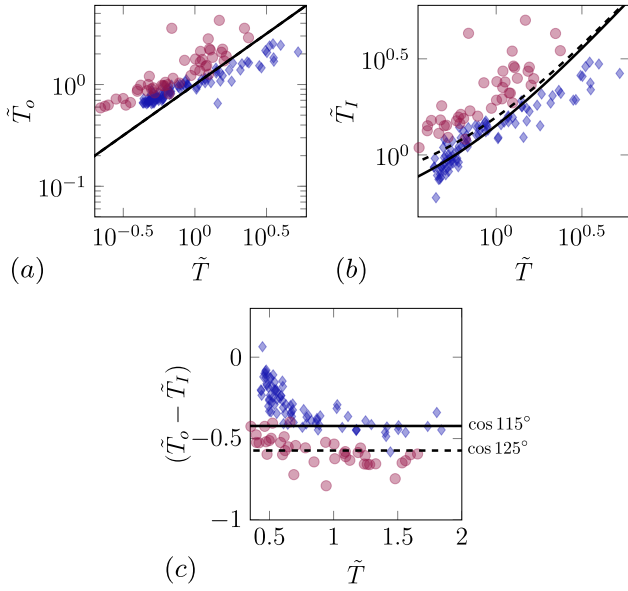
Fig. 4 (a) Non-dimensional applied tension \tilde{T}_o , (b) tension in the portion of the filament wet by the droplet \tilde{T}_l , and (c) the difference between these tension values, (\tilde{T}_o - \tilde{T}_l) evaluated by using angles \vartheta, \phi measured from experiments (using eqn. 5) as functions of the applied tension, \tilde{T} measured using soft-beam displacement. \circ correspond to filament diameter 205\mu\text{m} and \diamond to diameter 77\mu\text{m} for different droplet sizes. The solid and dashed lines respectively indicate theoretical predictions from eqn. 6.
