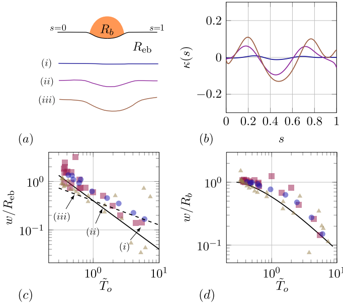
Fig. 5 (a) Three different filament shapes extracted from experiments as the applied tension T_o is decreased for a fixed droplet size of w = 6.2\text{mm} and filament diameter d = 120\mu\text{m} . (b) Corresponding signed curvature, \kappa(s) of shapes in (a) computed as a function of non-dimensional arc length s (scaled using filament length) after fitting Bezier spline to the extracted shapes. 1/R_{eb}, 1/R_b correspond to maximum and minimum of \kappa(s) . (c) The non-dimensional curvature of transition-zone close to the contact-line between filament and droplet, w/R_{eb} and (d) the non-dimensional curvature of the droplet wet part of filament, w/R_b as a function of non-dimensional boundary tension \tilde{T}_o for a filament of diameter d = 120\mu\text{m} for three different droplet sizes w = 6.2\text{mm} ( \Delta ), 7.6\text{mm} ( \circ ), 9.4\text{mm} ( \square ) and several values of T_o , non-dimensionalised using an estimate of \gamma = 5\text{mN/m} . The corresponding bendability values are \varepsilon^{-1} = 49, 72, 125 . The solid line in (c) corresponds to \tilde{T}_o^{-1} and the dashed line is \tilde{T}_o^{-1/2} while the solid line in (d) corresponds to the complete expression for \tilde{T}_o using eq. 8 for \varepsilon = 0 .
