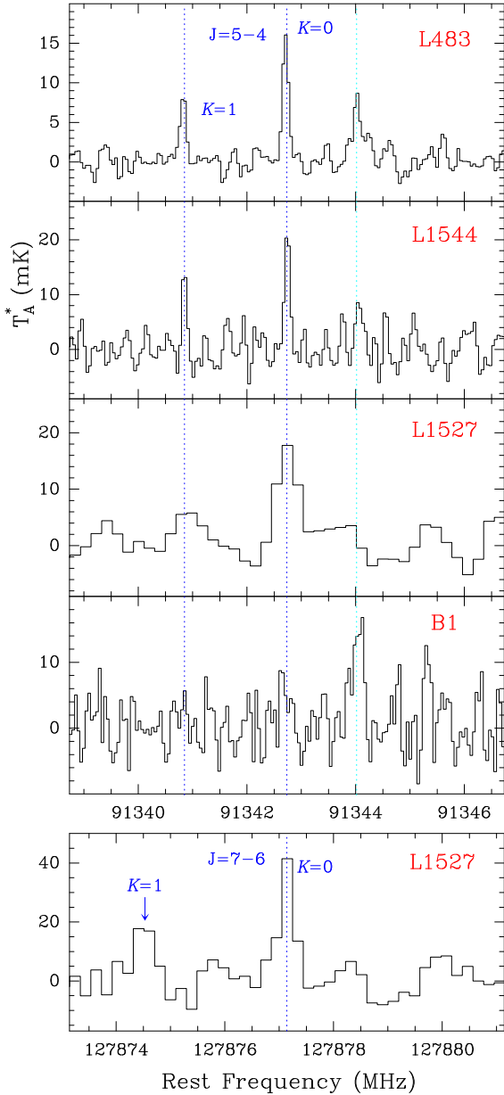
Fig. A.1. Observations of the J = 5 - 4 transition of CH 3 CO + towards L483, L1544, L1527, and B1 (top panels); bottom panel: J = 7 - 6 line towards L1527. The abscissa corresponds to the rest frequency (in MHz) and the ordinate is the antenna temperature (in mK). The spectral resolution is 48.8 kHz for all sources except L1527, for which it is 198 kHz. The vertical dashed blue lines indicate the position of the K = 0 and K = 1 lines (detected in all sources except B1), and the cyan line corresponds to the U feature at 91 344 MHz (detected in all sources except L1527). The rest velocities of L1527 and L1544 were taken as v_{\text{LSR}} = 5.9 \text{ km s}^{-1} and 7.2 \text{ km s}^{-1} , respectively, based on Sakai et al. (2009) and Vastel et al. (2015), respectively.
