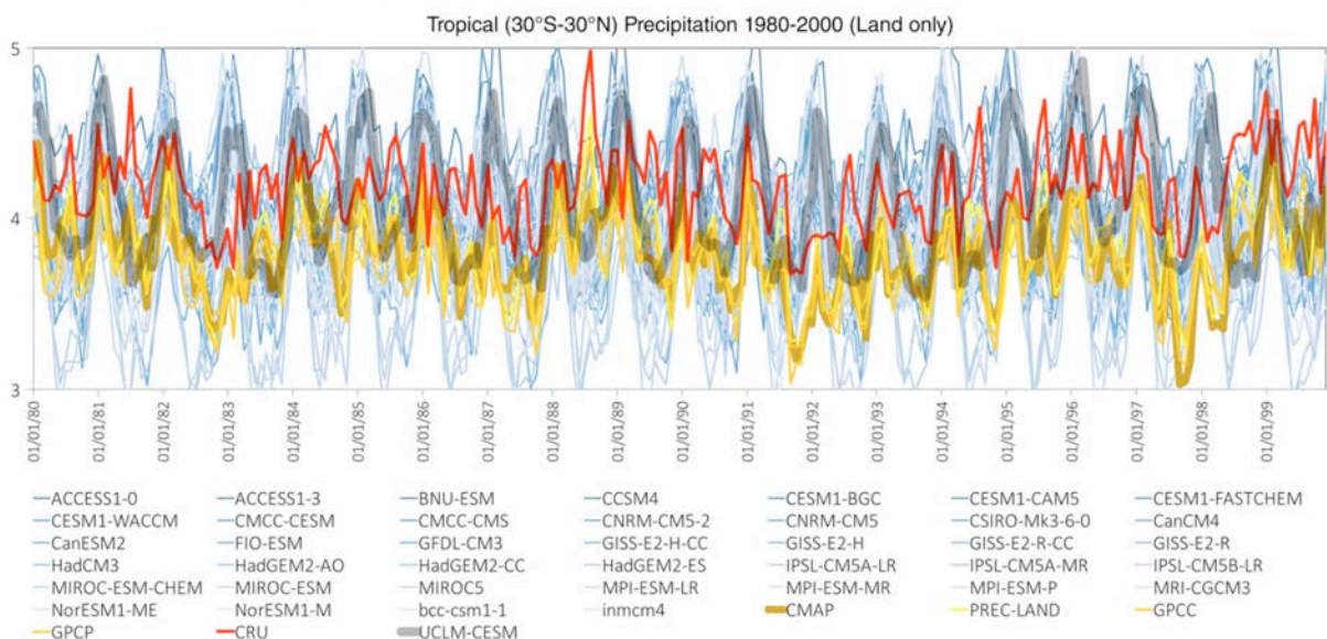
Figure 2.2.1. Time series of tropical ( 30\text{S} – 30\text{N} ) precipitation (mm/day) over land for 1980–2000. From Tapiador et al., 2018
