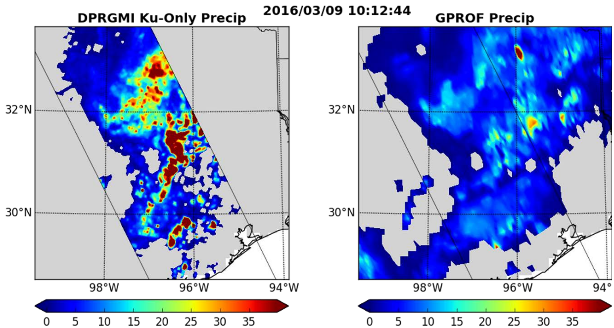
Figure 1.1.3. Side-by-side comparison of the precipitation estimate produced by the GPM combined DPR+GMI (CORRA) product (left panel), and the corresponding GMI-only (GPROF) estimate (right panel).
