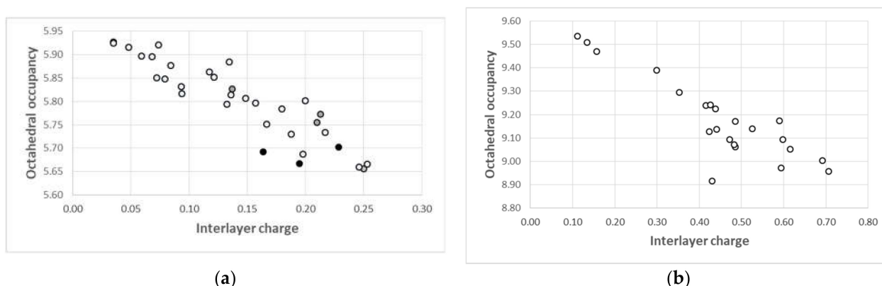
Figure 13. (a) Octahedral occupancies as a function of the interlayer charge for chlorite. Structural formulas are calculated per half formula unit (14 O). (b) Octahedral occupancies as a function of the interlayer charge for corrensite. Structural formulas are calculated per half formula unit (25 O). Black dot: compartment 1, white dot: compartment 2, grey dot: compartment 3.
