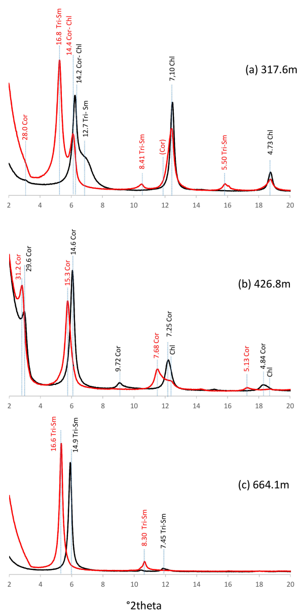
Figure 5. X-ray diffractograms of oriented preparations: infra 2 \mu\text{m} clay fraction. In black: air dried; and in red: ethylene glycol-solvated preparation. Tri-Sm: tri-smectite, Cor: corrensite, and Chl: chlorite.
