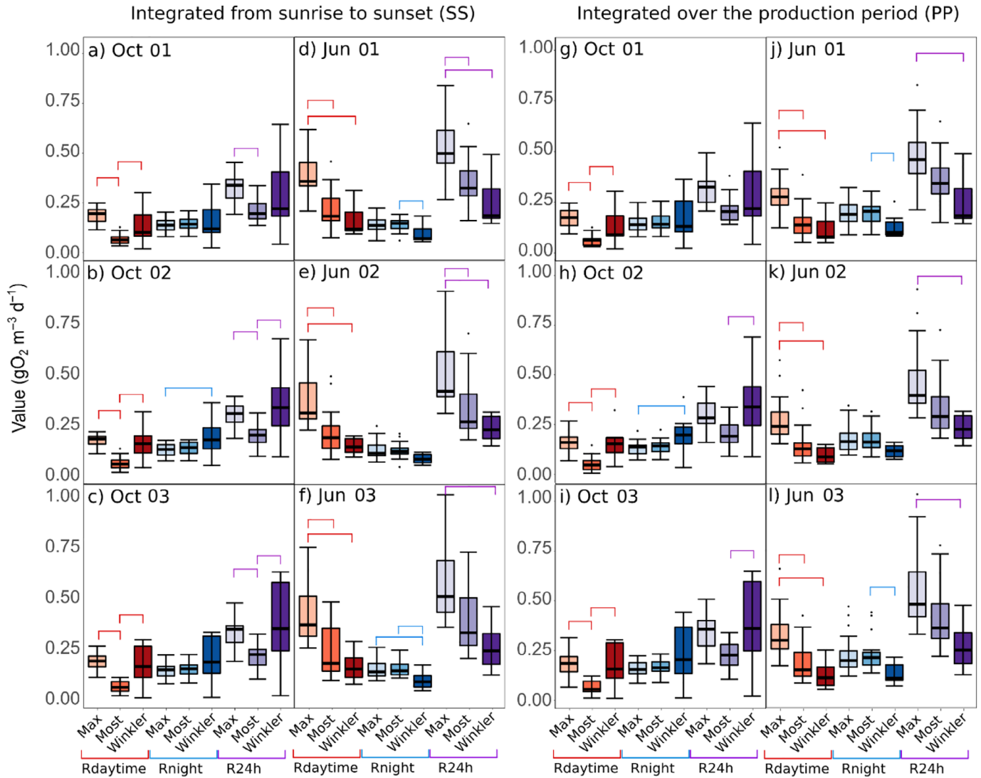
Fig 3. Estimates of R daytime (the three leftmost boxplots in orange), R night (the three boxplots in blue in the middle), and R (the three rightmost boxplots in purple) obtained from sensor data using the Max and Most methods and from Winkler incubation data integrated from sunrise to sunset or over the production period for Oct 01 (a, g), Oct 02 (b, h), Oct 03 (c, i), Jun 01 (d, j), Jun 02 (e, k), and Jun 03 (f, l). For each box, the lower quartile, median, and upper quartile values are displayed with horizontal lines. Whiskers show the range of the data, from the minimum to the maximum, excluding outliers. Brackets represent the comparisons between estimates that were found to be significantly different ( p < 0.05 , Tukey HSD or Dunn test). Oct 01, Oct 02, and Oct 03 refer to the mesocosms no.1, no.2, and no.3 of the October 2018 experiment, and similarly Jun 01, Jun 02, and Jun 03 refer to the mesocosms no.1, no.2, and no.3 of the May and June 2019 experiment.
