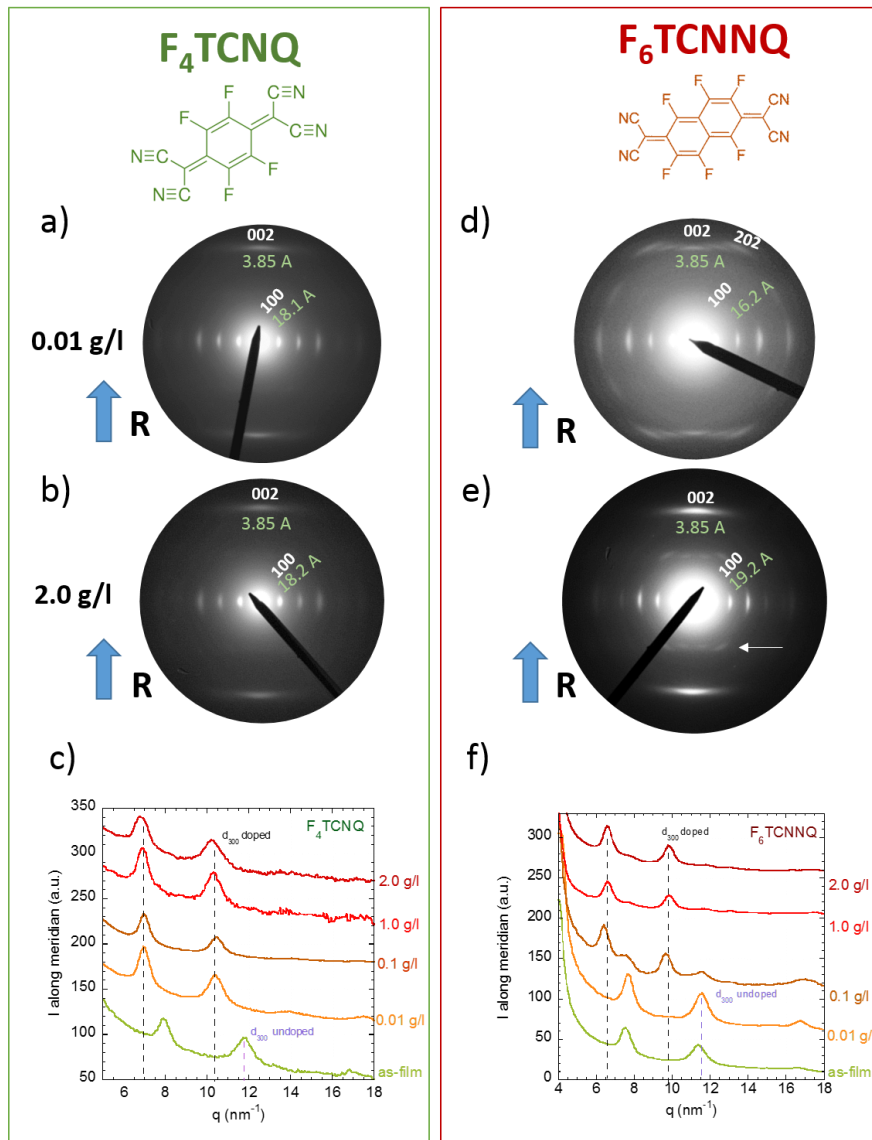
Figure 3: Electron diffraction patterns of oriented P3HT films doped with F_4TCNQ (a, b) and with F_6TCNNQ (d, e) for doping concentrations of 0.01 g/l (a,d) and 2.0 g/l (b, e), respectively. c) and f): equatorial section profiles of the electron diffraction patterns at different doping concentrations for F_4TCNQ (c) and for F_6TCNNQ (f). For clarity, the section profiles are shifted along the ordinate axis and the intensity of the patterns are normalized to the intensity of the 2 0 0 peak. The rubbing direction \mathbf{R} (blue arrow) is vertical for all patterns. The 0 0 2 reflection was used to calibrate the ED patterns. In the diffraction pattern (e), additional h 0 1 reflections related to the F_6TCNNQ -doped P3HT phase are indicated by a white arrow.
