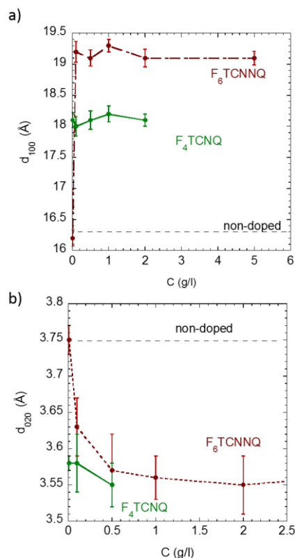
Figure 4: Evolution of the layer spacing along the alkyl side chain direction d_{100} (a) and the \pi -stacking periodicity (b) as a function of doping concentration. The curves in green (dark red) correspond to the F_4 TCNQ ( F_6 TCNNQ) doped films.
