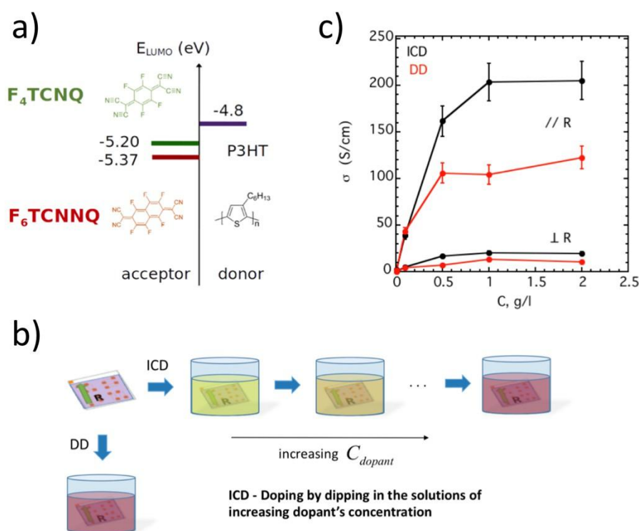
Figure 1. a) Energy diagram of the LUMO levels of F 4 TCNQ, F 6 TCNNQ and HOMO of P3HT, b) Schematic illustration of incremental concentration doping (ICD) and direct doping (DD) methods, c) Comparison of the electrical conductivity of oriented P3HT films doped with F 4 TCNQ in acetonitrile by the two doping methods as a function of increasing dopant concentration.
