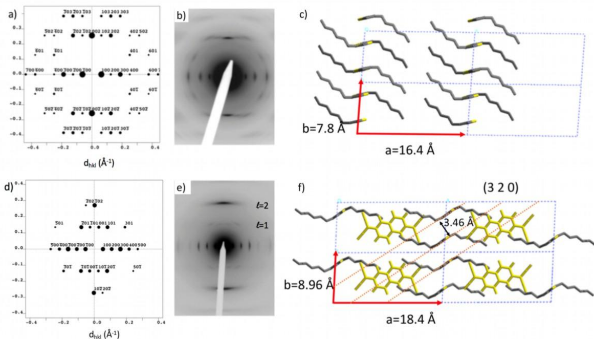
Figure 5. Calculated (a and d) and experimental (b and e) electron diffraction patterns for the [0\ 1\ 0] zone for P3HT (form I) (a and b) and P3HT- F_6 TCNNQ (d and e). The form I structure is taken from reference [30] whereas the doped P3HT structure is refined and corresponds to the model illustrated in Figure 6. In c) and f), the c -axis projection of the pristine and doped structures are shown, respectively.
