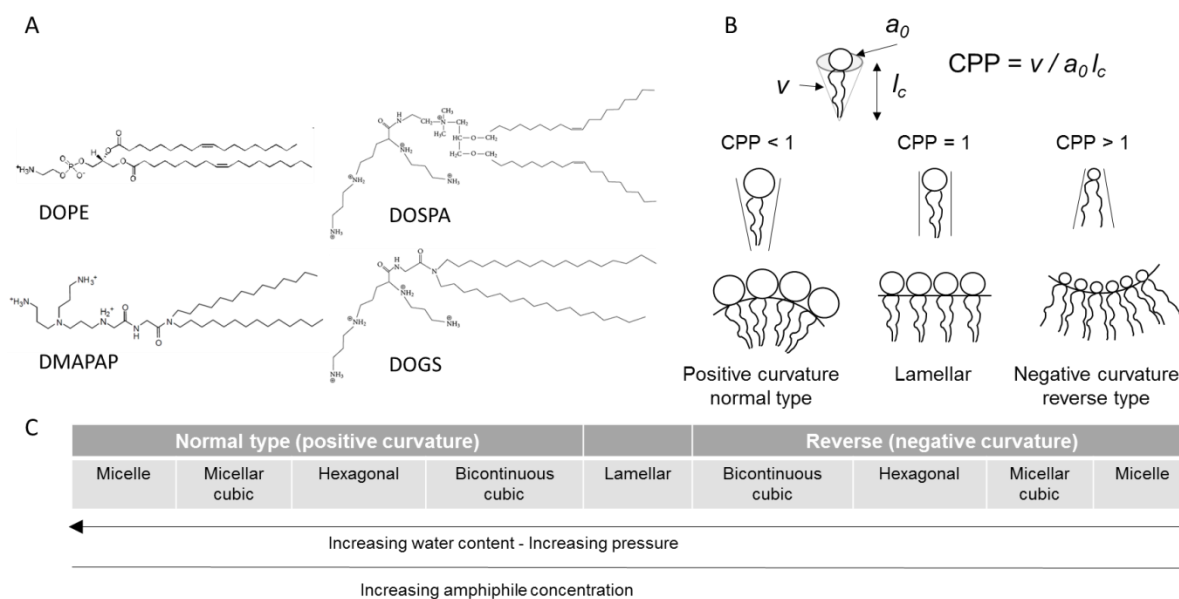
Figure 8. (A) Structure of cationic and zwitterionic lipids. DOPE = 1,2-dioleoyl-sn-glycero-3-phosphoethanolamine, DOSPA = 2,3-dioleoyloxy-N-(2(spermine carboxamido) ethyl)-methyl-1-propaniminium, DMAPAP = 2-{3-[Bis-(3-amino-propyl)-amino]-propylamino}-N-ditetradecylcarbamoyl methyl-acetamide, DOGS = dioctadecylamidoglycyl-spermin. (B) Molecular shapes and critical packing parameter (CPP) of amphiphiles and the structures formed. v = volume of hydrocarbon core, a_0 = effective head group area, l_c = hydrocarbon chain length. (C) Lyotropic liquid crystal phases (an ideal phase progression as a function of amphiphile concentration, pressure or water content in the system, from 58 ).
