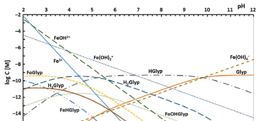
Fig. 2. Calculated speciation of 80 ng/L (0.47 nM) glyphosate in the presence of ferrihydrite, \text{FeOOH}_{(s)} , at 0.03 M ionic strength using VminteqA2 program (Glyp represents the most deprotonated species of glyphosate). Stability constants for glyphosate complexation with Fe(III) are from Motekaitis and Martell (1985) [46].
