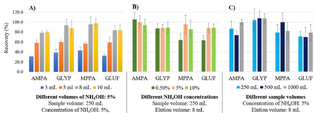
Fig. 3. Evaluation of one-step extraction procedure by determination of mean recoveries of the four target compounds in the function of the differences of ammonium extraction volume (A), ammonium concentration (B), and sample volume (C) at spiked 80 ng/L concentration in sea water. Five replicated experiments were implemented for each condition.
