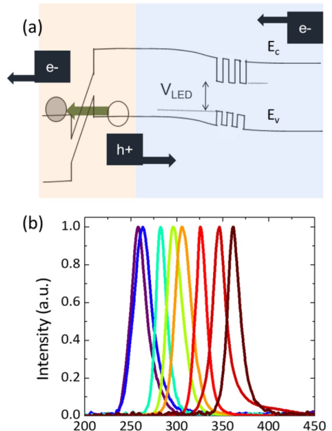
Figure 29. (a) Schematic energy band diagram of a tunnel-injected UV LED structure under forward bias. (b) Summary of the emission spectra achieved in tunnel-injected UV LEDs. Reprinted with permission from [187]. Copyright (2018), AIP Publishing LLC.
