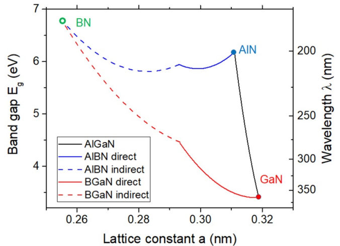
Figure 13. Bandgap versus lattice constant of the ternary alloys BGaN and AIBN. Notice the indirect band structure of w-BN. The connecting lines are plotted as a best compromise of unfortunately not yet fully consistent data from several sources. The direct band gap of w-BN is taken as 10.2 eV [85], whereas bowing parameters of 7 and 4 eV are assumed for the direct (full lines) and indirect transitions (broken lines), respectively, for both B-containing ternaries. For simplicity we assumed Vegard's law for the lattice constant. Any slight deviation (as sometimes discussed) would not change the major message of this diagram.
