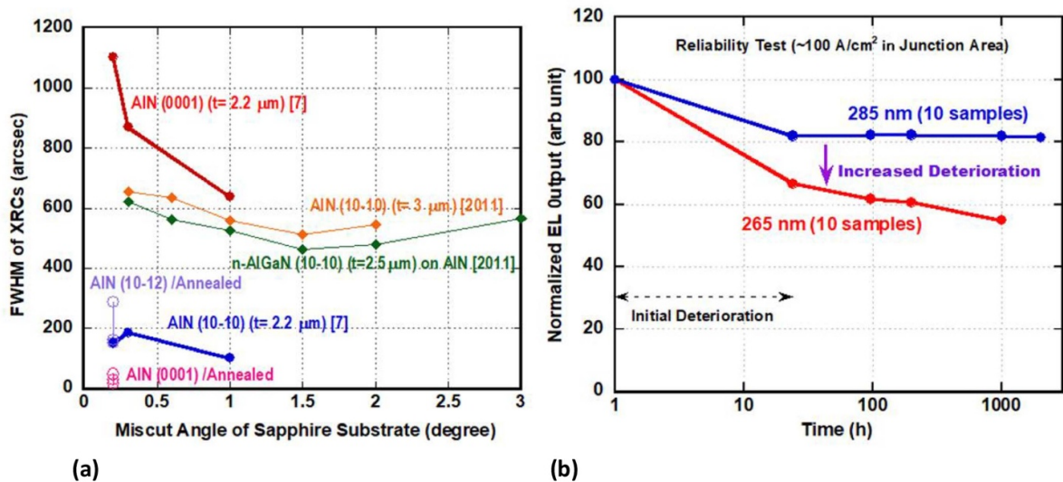
Figure 19. (a) Full width at half maximum (FWHM) of XRCs for AlN template and AlGaIn layer on AlN template and (b) result of the reliability test for 265 nm LEDs. In (a), the improvement in XRCs using sapphire substrates with high miscut angles is shown. Recently reported FWHMs of XRCs obtained using a sputtered AlN film on sapphire followed by annealing have also been added (hollow symbols), showing the possible improvement in IQEs, which is considered to be useful for examining the possible improvement. Reproduced from [114]. © 2020 The Japan Society of Applied Physics. All rights reserved.
