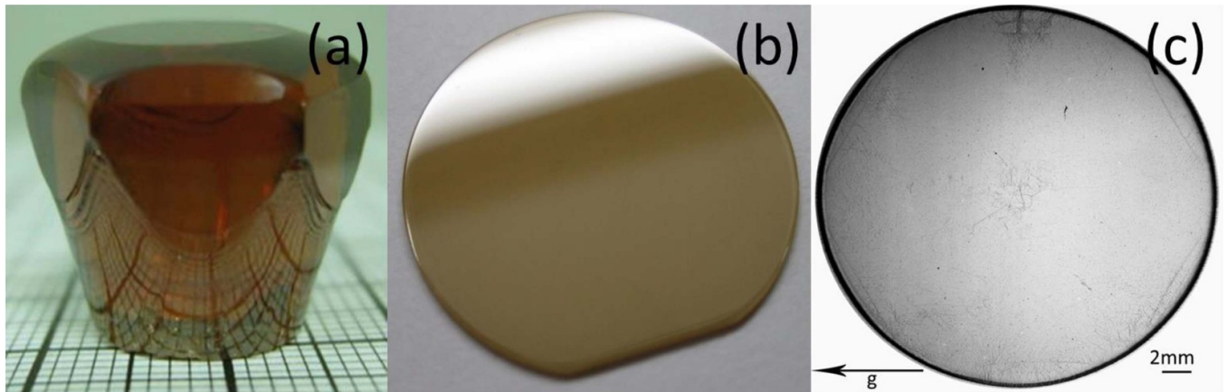
Figure 4. (a) Photograph of an AlN boule grown via the PVT method (mm-grid); (b) image of a 1" AlN wafer after mechanical and chemo-mechanical polishing; (c) x-ray topograph confirming that most of the wafer area is dislocation free.
