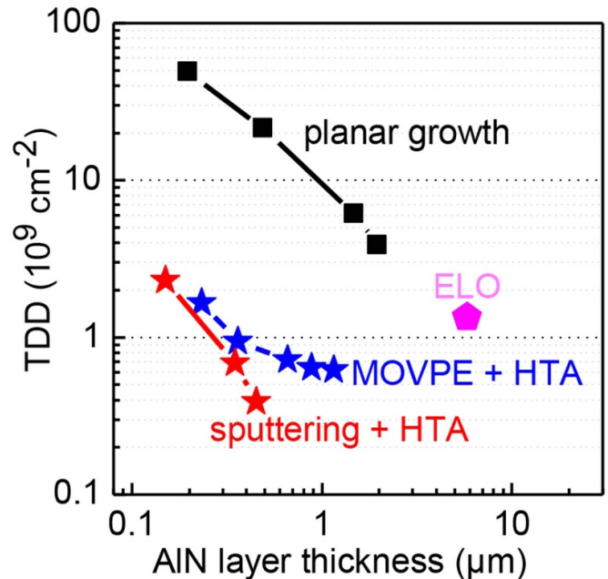
Figure 3. Reduction of threading dislocation density with grown AlN layer thickness. For planar growth, cracking limits the thickness that can be achieved. Epitaxial lateral overgrowth (ELO) patterning allows thicker layers and thus lower TDD but is not very economic [10]. High temperature annealing (HTA) achieves low TDD already for much thinner layers. (S Hagedorn et al. , Ferdinand-Braun-Institut, unpublished results.)
