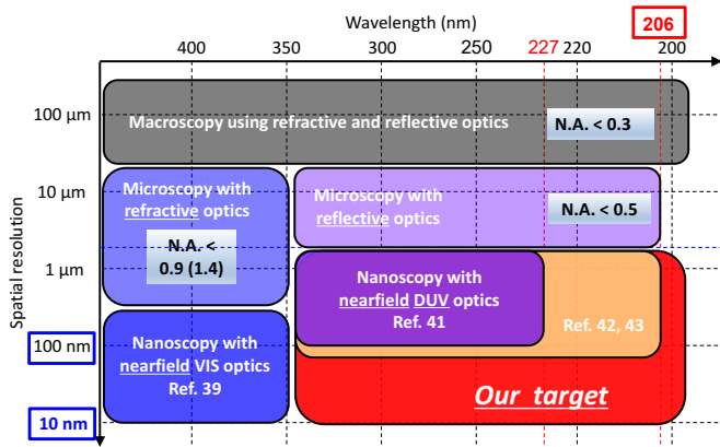
Figure 7. Current status and future prospect of PL-mapping technology.
