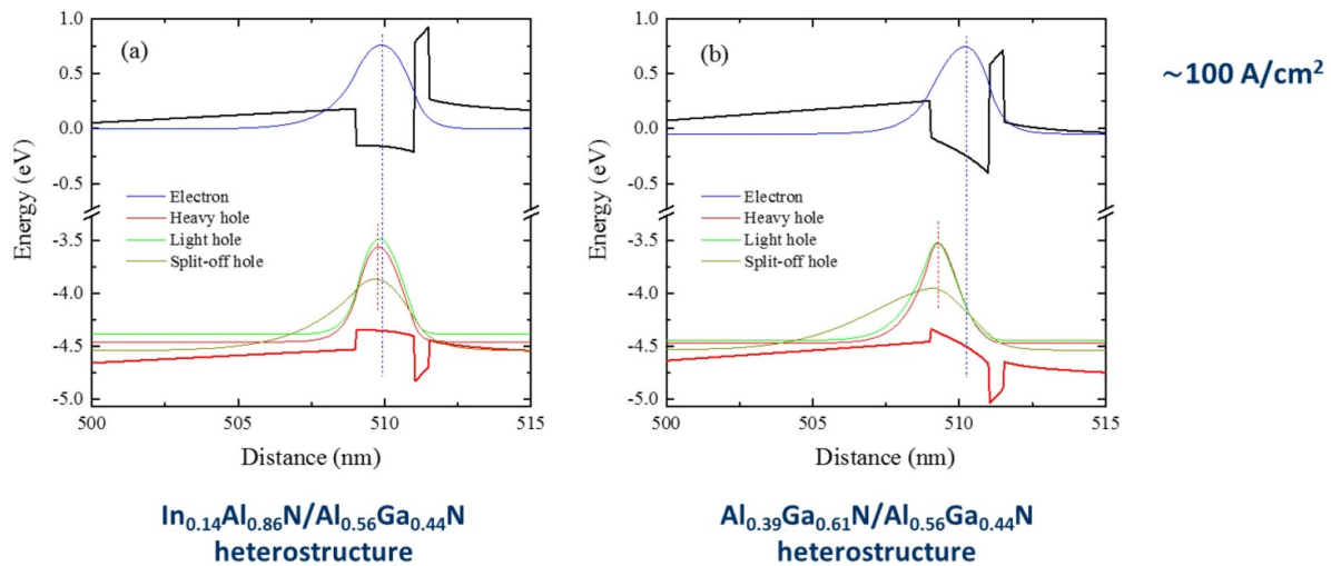
Figure 16. Improved electron–hole wavefunction overlap for InAlN–AlGaN versus AlGaN–AlGaN quantum well UVA LEDs ( \sim 340 nm). Reproduced from [109]. © 2019 The Japan Society of Applied Physics. All rights reserved.
