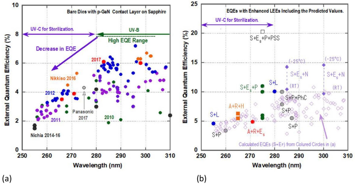
Figure 18. (a) EQEs from various groups for dies with p-GaN contact layer on sapphire. Coloured data are the results obtained at UV Craftory. (b) Initial EQEs of UV-LEDs with roughening (+R), with encapsulation (+E), with a sapphire lens (+L), with a p-reflective contact (+P), with an n-reflective electrode (+N), and with the use of a PSS (+PSS). The subscripts ‘S’ and ‘F’ after ‘+E’ indicate unknown/or silicone and fluoro-resin, respectively. ‘A’ and ‘S’ denote sapphire and AlN bulk substrates, respectively. The regrowth of an AlN layer with UVC transmittance by HVPE on an AlN substrate followed by removing the AlN bulk substrate is indicated as (+H). The data in (b) are limited to those published later than 2013. Also, the calculated achievable EQEs are shown by hollow symbols. Our calculated data for the case of fluoro-resin encapsulation from the data in (a) are indicated by hollow violet, and the solid violet is based on the experiment. In the graphs, data for 280–310 nm UVB-LEDs show the lower EQEs for UVC (250–280 nm). The EQE in UVC is considered to be suppressed by the decreases in IQE and CIE. Reproduced with permission from [122].
