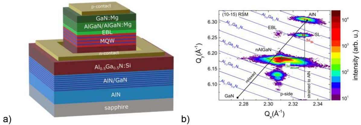
Figure 17. (a) Schematic of a typical UVB-LED heterostructure. For coherent growth of the MQW emitting at 305 nm a relaxed \text{Al}_{0.5}\text{Ga}_{0.5}\text{N} layer is grown (from Susilo et al. , pssa). (b) XRD reciprocal space map around the AlN 105 reflection of a full UVB LED illustrating the strain relaxation process. The AlN/GaN superlattice is grown coherently strained on the AlN/sapphire template (nearly the same Q_x value). The \text{Al}_{0.5}\text{Ga}_{0.5}\text{N} starts to grow first strained but then relaxes during further overgrowth ( Q_x shifting to lower values) thus forming a metamorphic quasi-substrate that allows to grow EBL and buffer layer with the new lattice constant. Reprinted from [113], Copyright (2017), with permission from Elsevier.
