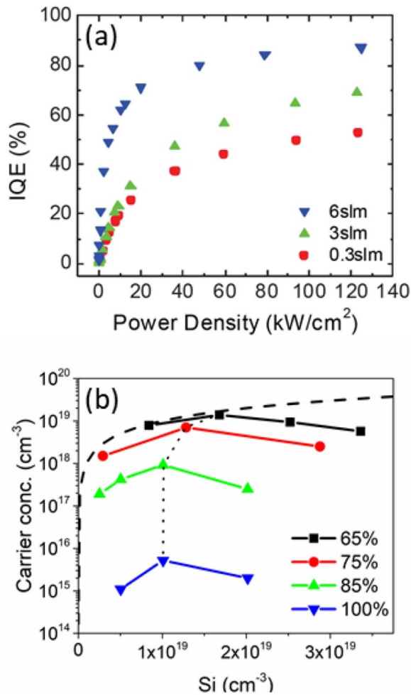
Figure 8. (a) The IQE for AlGaIn MQW structures on single crystal AlN substrates as a function of excitation power density shown for different point defect concentrations (here, higher ammonia flow corresponds to lower non-radiative recombination defect centre concentrations). (b) The dependence of carrier concentration as a function of doping concentration for different Al compositions in the alloy AlGaIn. The black dashed line assumes the carrier concentration to be same as silicon concentration.
