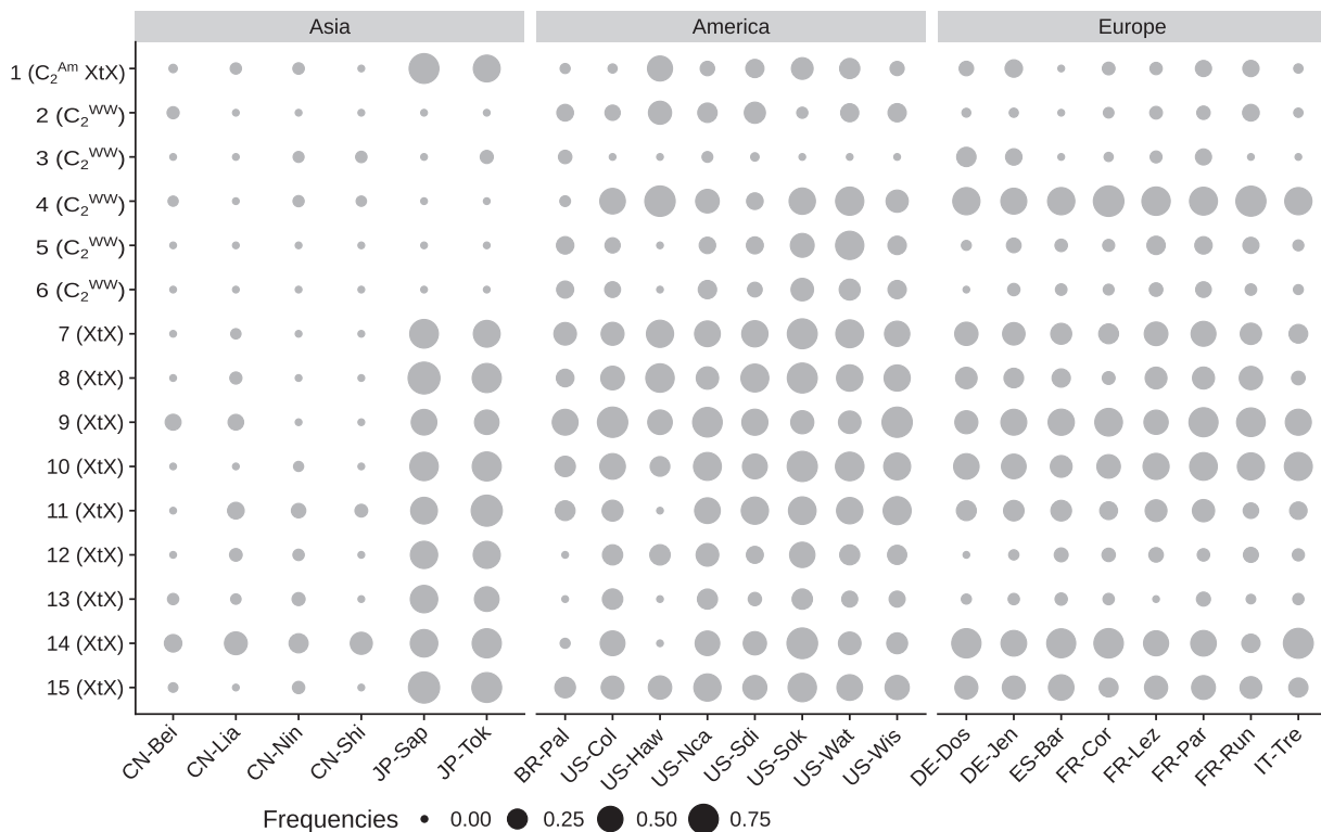
FIG. 4. Frequencies of each of the 15 putatively adaptive insertions in the 22 Drosophila sukuzii populations. Insertion number is indicated on the left together with the associated BayPass statistics. XtX corresponds to a global differentiation statistic, C_2 to a statistic contrasting allelic frequencies between native populations and populations of the invasive American road ( C_2^{Am} ) or populations of the invasive European road ( C_2^{Eu} ) or all invasive populations ( C_2^{WW} ).
