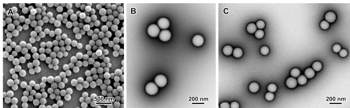
Figure 5. SEM (A) and TEM (B,C) images of PSTY (A,B) and PMMA (C) nanoparticles prepared in the presence of 8 wt% dextrans at 30 wt% SC. In B and C, the preparations have been negatively stained with uranyl acetate.
