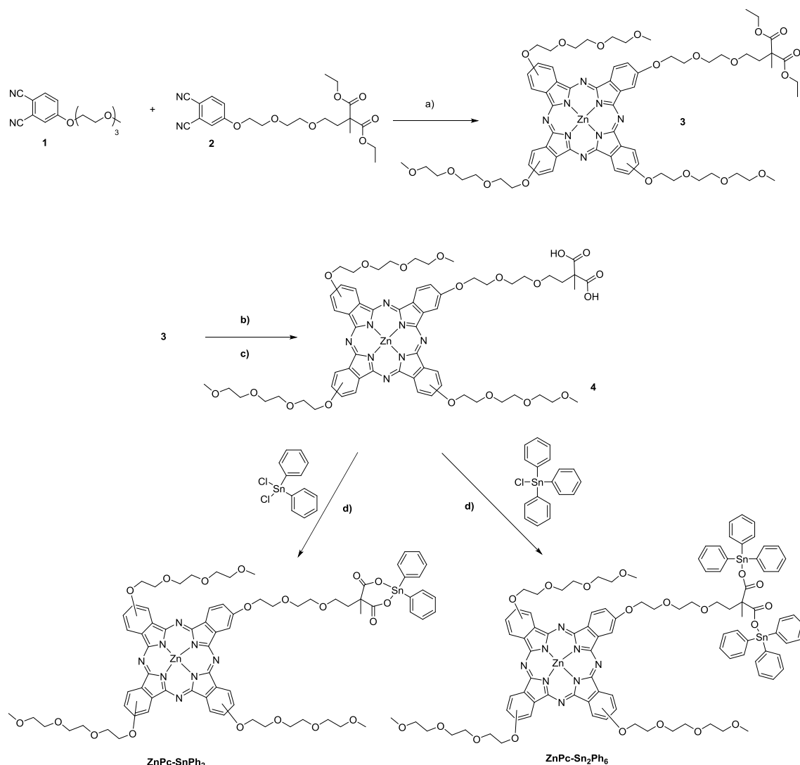
Scheme 1. Synthetic route for the preparation of the dyads composed of a zinc phthalocyanine linked to a tin complex. Reagents and conditions: (a) n-pentanol, DBU, \text{Zn}(\text{OAc})_2 \cdot 2\text{H}_2\text{O} , 140-150°C, 12 h, 18% ; (b) acetone, NaOH, reflux, 2 h ; (c) HCl, 85%; (d) THF, TEA, room temperature, 12 h, 100%.
