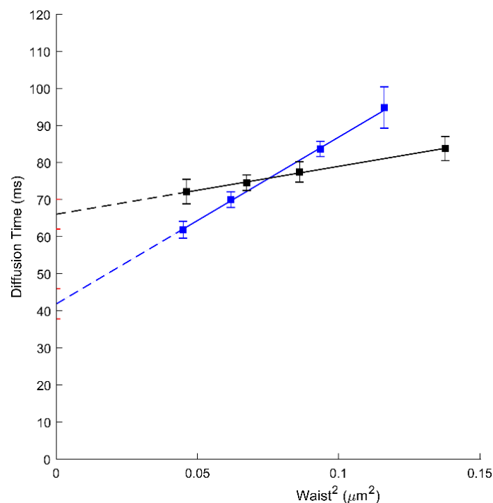
Figure 2. svFCS diffusion laws for an active ABCA1 in non-treated A1G cells (black) and after ApoA1 binding (blue).
