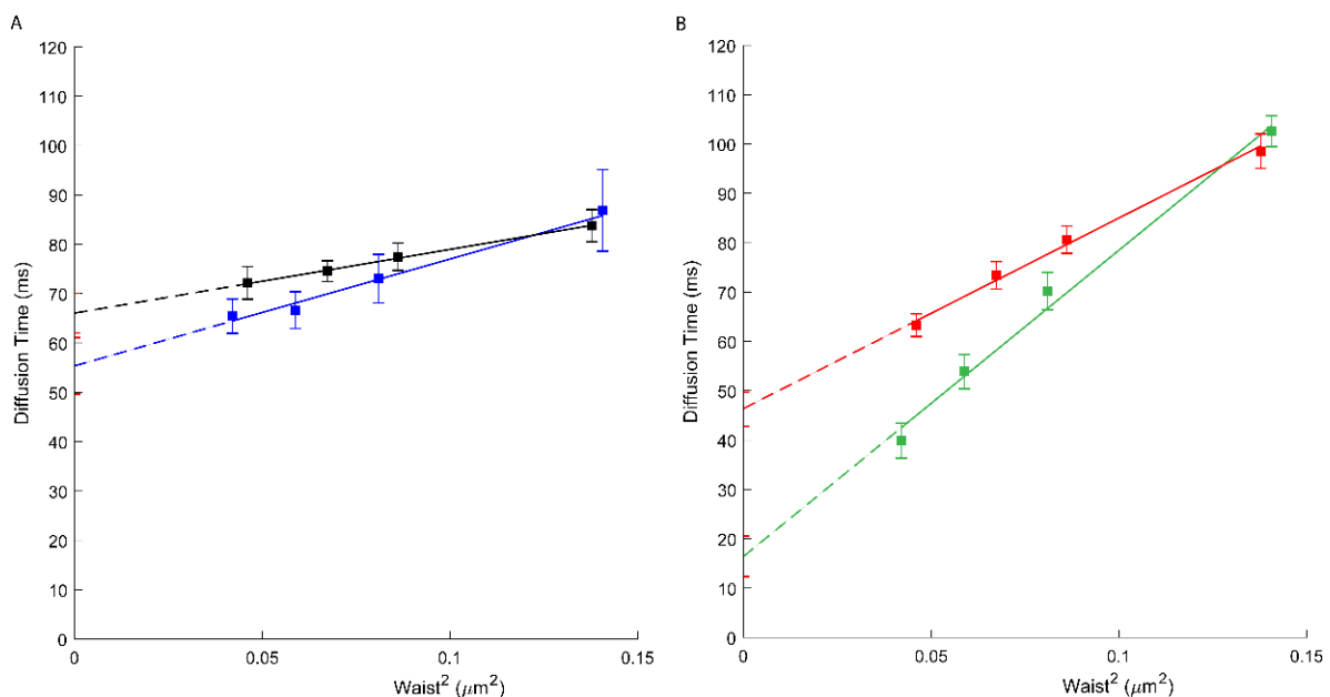
Figure 1. (A) svFCS diffusion laws for an active ABCA1 in non-treated A1G cells (black) and after amphotericin B treatment (blue). (B) svFCS diffusion laws for a non-active ABCA1MM in non-treated MMG cells (red) and after amphotericin B treatment (green).
