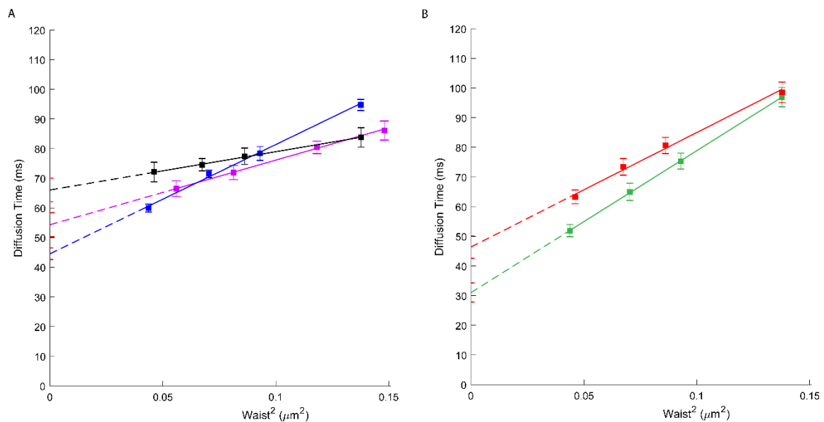
Figure 3. (A) svFCS diffusion laws for an active ABCA1 in non-treated A1G cells (black), after cholesterol oxidase treatment (blue) and after reload with cholesterol-methyl- \beta -cyclodextrin (violet). (B) svFCS diffusion laws for a non-active ABCA1MM in non-treated MMG cells (red) and after cholesterol oxidase treatment (green).
