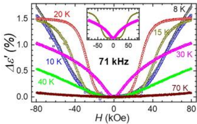
FIG. 4. Fractional change of dielectric constant as a function of magnetic field at selected temperatures and a fixed frequency of 71 kHz. The inset is an enlargement of \Delta\epsilon_0 vs H at 15 and 30 K in order to highlight the change of shape around 20 kOe.
