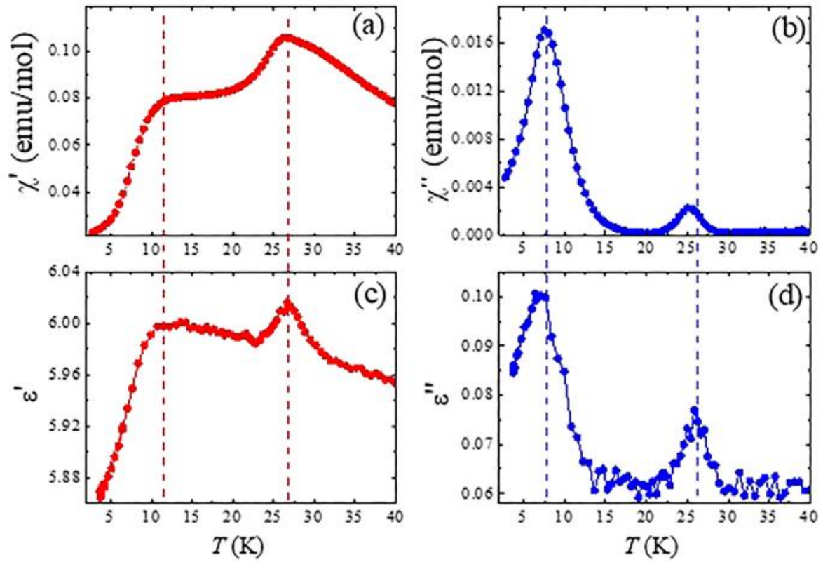
FIG. 3. In-phase (a) and out-of-phase (b) magnetic susceptibility recorded in 1 T at a frequency of 10 kHz. In-phase (c) and out-of-phase (d) dielectric constant recorded in the same magnetic field and at a very close frequency (11.1 kHz). The dashed lines show the correspondences between the magnetic and dielectric data.
