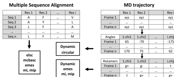
Fig. 1. Schematic representation of the correlation/covariation analyses provided by the Bios2cor package.
