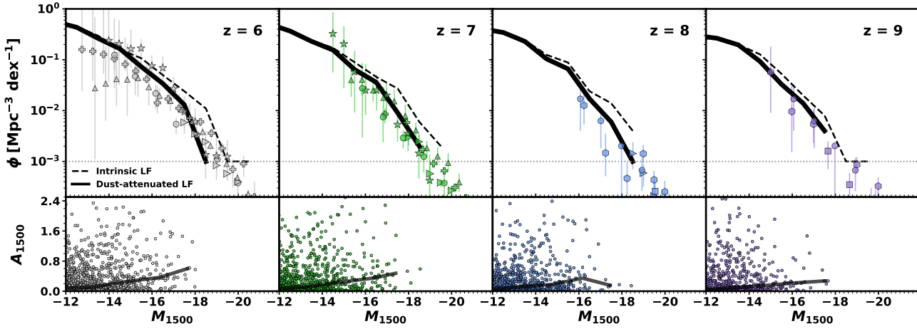
Figure 4. UV luminosity functions (LF; 1500 Å rest-frame) at z = 6, 7, 8 and 9 (top). The dashed and solid black curves correspond to the intrinsic and dust-obscured LFs respectively. We compare with observations represented by the symbols: Bouwens et al. (plus signs 2015, 2017), Bhatwdekar et al. (circles 2019), Finkelstein et al. (right triangles 2015), Livermore et al. (2017, stars), Atek et al. (2015, 2018, upward triangles), Ishigaki et al. (hexagons 2018), and Oesch et al. (squares 2013). The data points of Atek et al. are shifted by -0.1 mag for clarity. The grey horizontal dotted line indicates our volume limit of one object per bin. We also show the dust attenuation, A_{1500} , as a function of UV magnitude (bottom). Dots correspond to individual galaxies and the line shows the median A_{1500} per M_{1500} bin.
