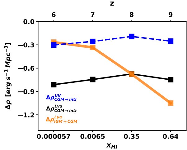
Figure 8. Evolution of the Ly \alpha and UV luminosity density decrement as a function of the IGM neutral fraction, x_{HI} . The top x-axis shows the redshifts of the corresponding snapshots of the SPHINX simulation. The Ly \alpha and UV density have been integrated down to L_{Ly\alpha} = 10^{40} erg s ^{-1} and M_{1500} = -12 respectively which approximately corresponds to our completeness limit.
