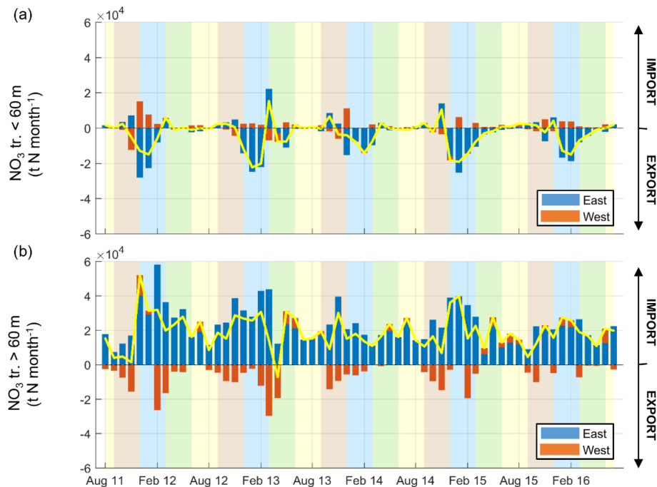
Figure 8. (a) Temporal variability of the monthly net surface (depths < 60 m) transport of NO 3 (tN per month) through the sections defined in Fig. 1. By convention, import (export) of NO 3 is shown by positive (negative) values. The residual net transport is shown by the yellow line. Shaded areas show the different seasons over the period simulated (yellow, JJA; brown, SON; blue, DJF; green, MAM). (b) Same as (a) but for depths > 60 m.
