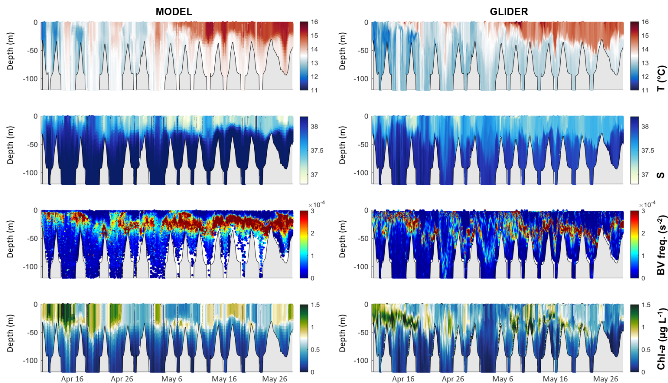
Figure 5. Comparisons of model outputs (left) and glider-based measurements (right) of (from top to bottom) temperature (°C), salinity, derived Brunt–Väisälä frequency ( \text{s}^{-2} ), and chlorophyll a ( \mu\text{g L}^{-1} , corrected from quenching for glider data). Simulated data correspond to the extracted data at the glider time and position. Bathymetry is shown in grey.
