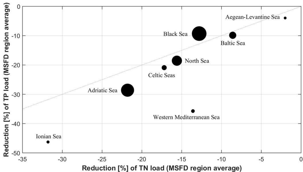
FIGURE 5 | Relative change of chlorophyll-a concentration per MSFD region (only ensemble means; symbol size refers to the change intensity of chlorophyll-a) as function of the reduction of the riverine TN and TP inputs.
