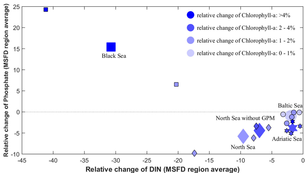
FIGURE 6 | Relative change of chlorophyll-a concentration per MSFD region (bluish colors refer to the change intensity of chlorophyll-a) as function of the relative changes of the dissolved nutrients DIN and phosphate from all the single models (ensemble means per region are highlighted by the enlarged symbols).
