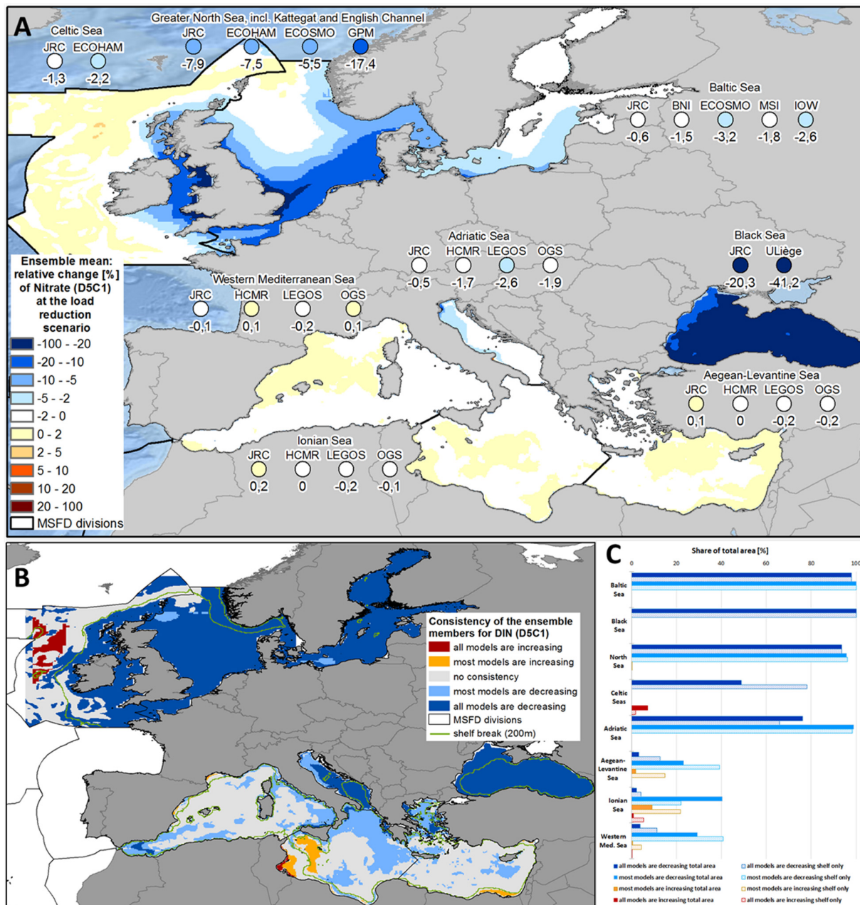
FIGURE 2 | (A) Ensemble means and model-specific relative change at load reduction scenario (compared to reference scenario) for the MSFD regions of nitrate (MSFD indicator D5C1). (B) Consistency map showing, if all or at least most models have the same trend of the relative change at load reduction scenario (compared to reference scenario) with respect to nitrate (MSFD indicator D5C1). (C) Share of the total area (bold bars) and of the shelf region (dotted bar), where all or most models show consistent changes with respect to nitrate (MSFD indicator D5C1).
