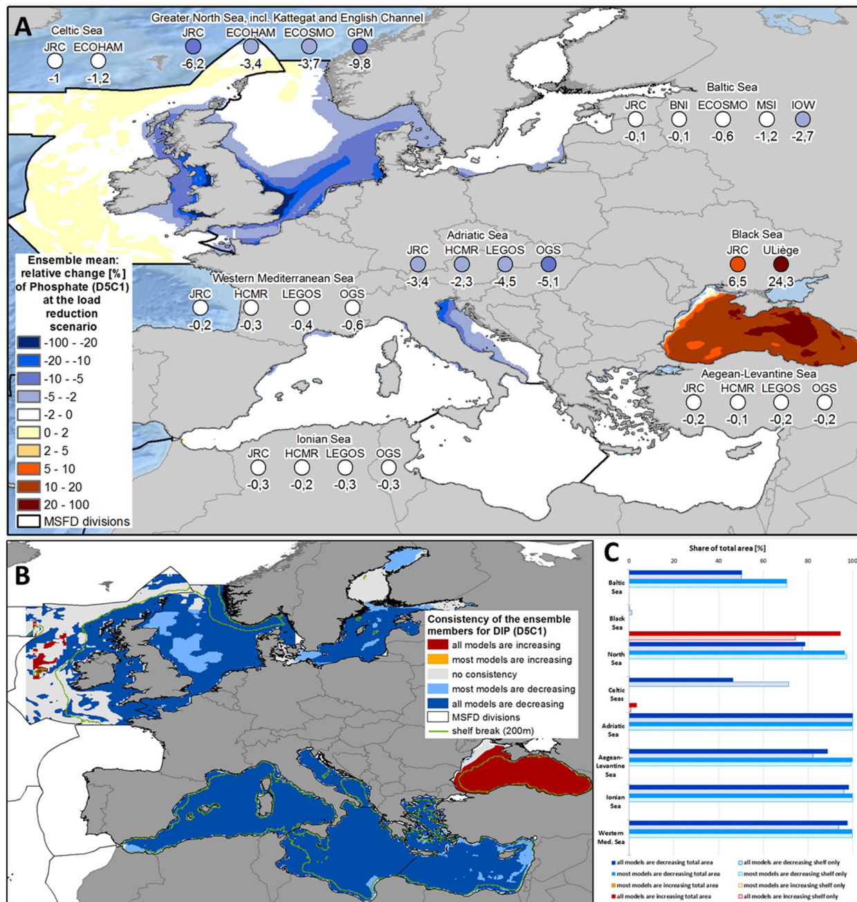
FIGURE 3 | (A) Ensemble means and model-specific relative change at load reduction scenario (compared to reference scenario) for the MSFD regions of phosphate (MSFD indicator D5C1). (B) Consistency map showing, if all or at least most models have the same trend of the relative change at load reduction scenario (compared to reference scenario) with respect to phosphate (MSFD indicator D5C1). (C) Share of the total area (bold bars) and of the shelf region (dotted bar), where all or most models show consistent changes with respect to phosphate (MSFD indicator D5C1).
