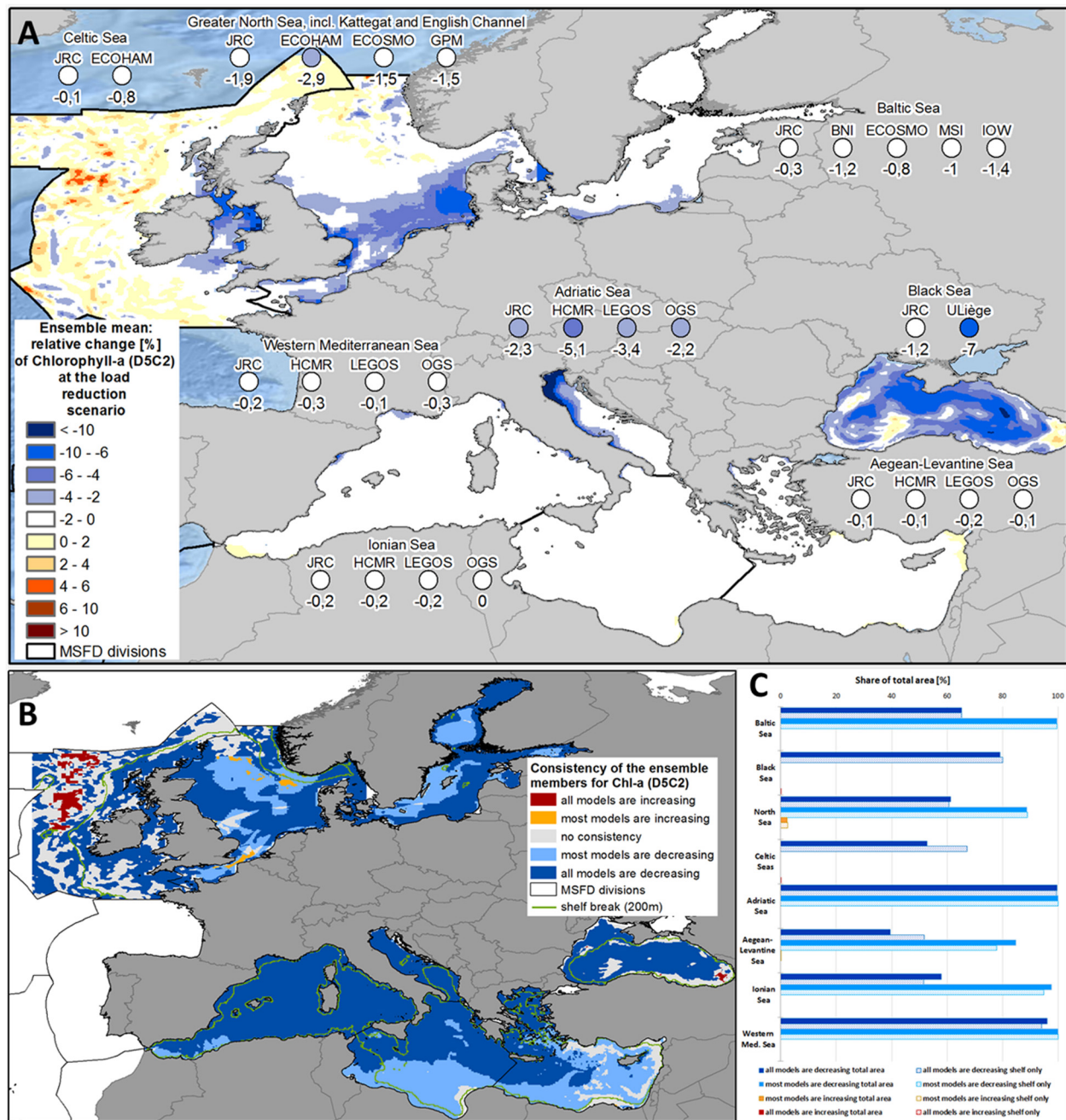
FIGURE 4 | (A) Ensemble means and model-specific relative change at load reduction scenario (compared to reference scenario) for the MSFD regions of chlorophyll-a (MSFD indicator D5C2). (B) Consistency map showing, if all or at least most models have the same trend of the relative change at load reduction scenario (compared to reference scenario) with respect to chlorophyll-a (MSFD indicator D5C2). (C) Share of the total area (bold bars) and of the shelf region (dotted bar), where all or most models show consistent changes with respect to chlorophyll-a (MSFD indicator D5C2).
