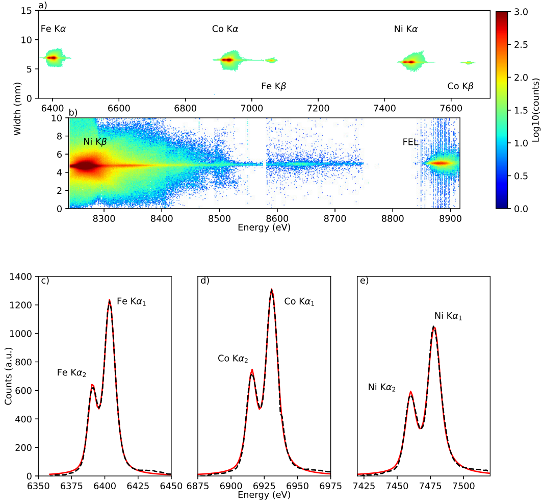
Figure 3. Spectra taken with two spectrometers employing R = 50 mm HAPG crystals. Above a) shows the forward-scattering spectrometer with emission lines from Fe, Co, and Ni. In b) we show the backward-scattering spectrometer with Ni K \beta and the FEL labelled. The colour scale is logarithmic and corresponds to both figures — white corresponds to zero counts. Below: lineouts (black dashed) from the image shown in a). Left c) shows the Fe K \alpha doublet fitted (in red) with the sum of two Pseudovoigt profiles. Similarly in d) (centre) and in e) (right) the Co K \alpha and Ni K \alpha doublets are shown fitted (in red).
