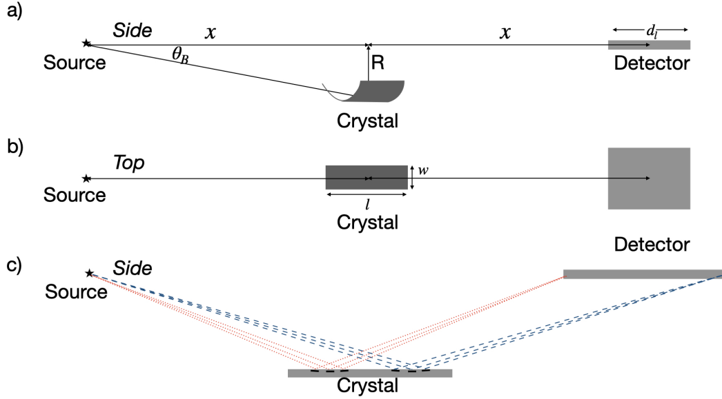
Figure 1. Schematic setup of a spectrometer in von Hámós geometry viewed from the side a) and from the top b). The crystal is located at a linear distance x from the source, as is the detector from the crystal. The cylindrically bent crystal is offset from the source-detector ( 2x ) line by its radius-of-curvature ( R ) making a Bragg angle of \theta_B to the source-detector line resulting in focussing in the non-dispersive axis. The crystal has a width w and a length along its cylinder axis of l . The detector chip has length along the dispersive direction of d_l . Also shown in c) is an example of mosaic focussing (not to scale) viewed from the side: red dotted is the lowest energy recorded on the detector and blue dashed is the highest energy.
