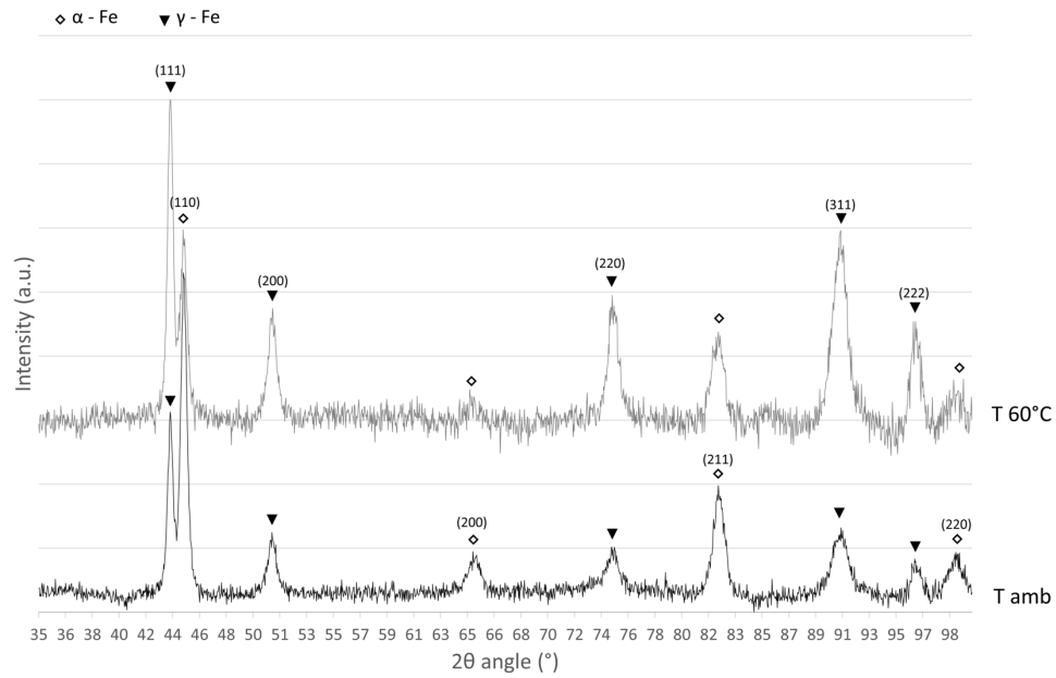
Figure 13: X-ray \theta - 2\theta background subtracted spectra of the fracture surface of the 316L steel (ambient T^{\circ} and 60^{\circ}\text{C} )
