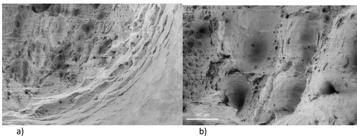
a) b) Figure 8: 316L-eGaln tested at room T° and 8.33 \times 10^{-5} \text{ m.s}^{-1} . a) low magnification of the fracture surface and b) close view of the crack initiation site on the left of a).
