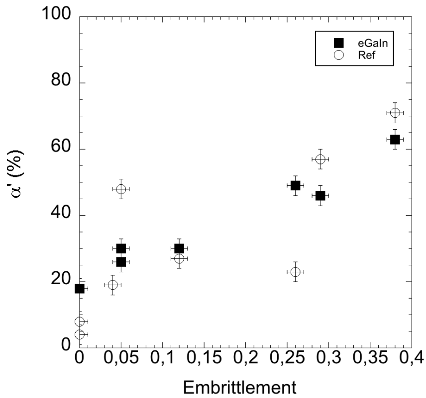
Figure 16: Correlation between degree of embrittlement and α' phase fraction for Galn tested samples with varying temperatures [RT,110°C]
