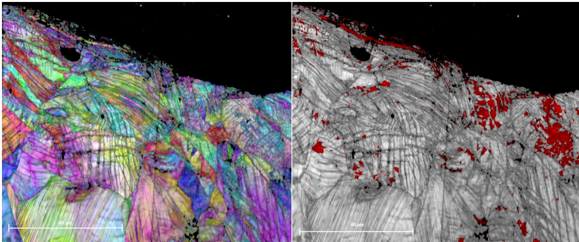
Figure 12: EBSD mapping of a transverse cut below fracture surface of 316L fractured in eGaln at a temperature of 75°C and 8.33 \times 10^{-7} \text{ m.s}^{-1} cross-head speed a) crystalline orientation + IQ b) phase map + IQ ( \alpha' in red)
