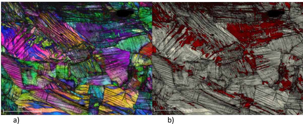
a) b) Figure 10: EBSD mapping of a transverse cut below fracture surface of 316L fractured in eGaln at room temperature and 8.33 \times 10^{-7} \text{ m.s}^{-1} cross-head speed a) crystalline orientation + IQ b) phase map + IQ ( \alpha' in red)
