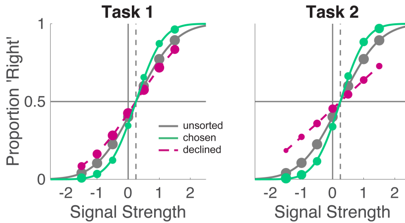
Figure 16. Effect of confidence bias on the psychometric functions. In these simulations, the first task was properly scaled ( \beta = 1.0 ) but the observer was over-confident in the second task ( \beta = 2.0 ). As a result, whenever task 1 is competing with task 2 in a confidence pair, confidence choice is biased in favor of task 2 (indicated by larger green dots for task 2 than for task 1). All parameters except \beta are identical across the two tasks and listed in Table 2. Plotting conventions are the same as those used in Figure 2B.
