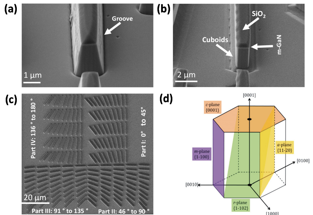
Figure 2. SEM images of fingers after GaN etching; (a) bird eye view of finger after dry etching; (b) bird eye view of finger after wet etching with TMAH solution; (c) top view of an ensemble of fingers for orientation between 0° and 180°; (d) GaN crystallographic planes [33].
