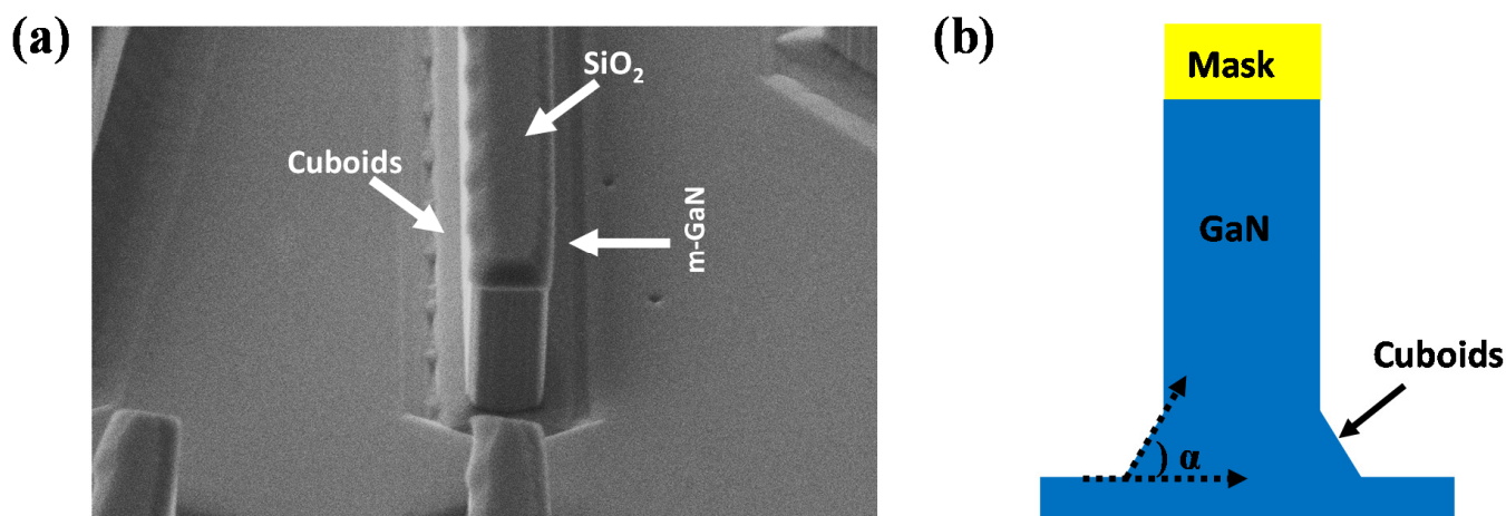
Figure 4. Groove formation due to the GaN etching; (a) This work; (b) description of cuboids formation.
