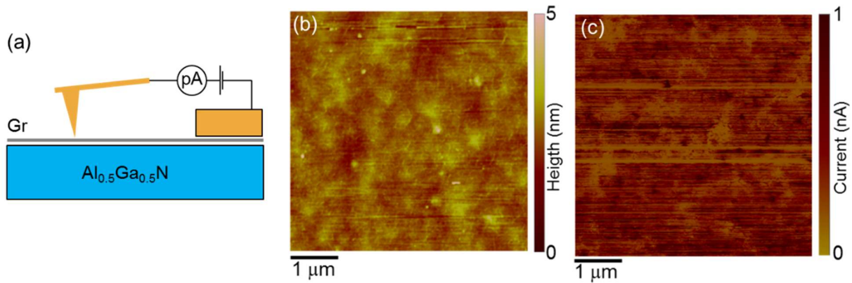
Figure 8. (a) Schematic of the experimental setup for C-AFM measurements on CVD grown graphene on AlGaN. Representative morphology (b) and current map (c) measured on the graphene surface by applying a tip bias of 100 mV.
