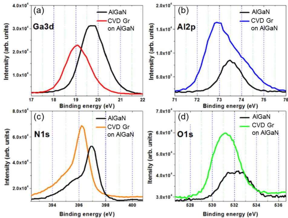
Figure 5. (a) Ga3d, (b) Al2p, (c) N1s and (d) O1s core-level peaks for the pristine AlGaN sample and after CVD with 3.5 sccm \text{C}_3\text{H}_8 at 1350°C under 10 slm of \text{N}_2 at 800 mbar.
