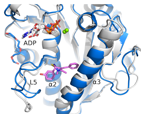
(R)-monastrol-97
