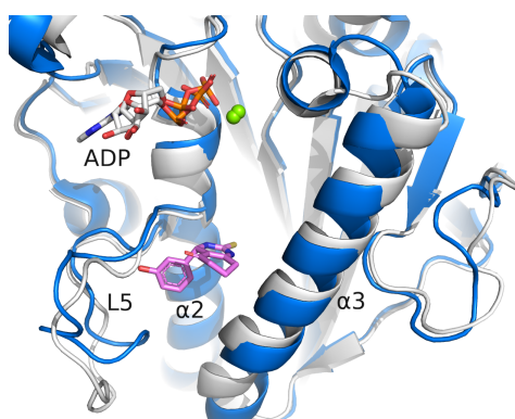
(S)-enastron
