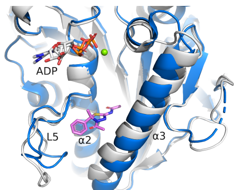
K858
