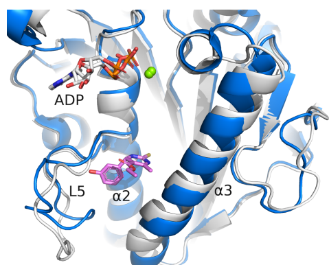
Monastrol
