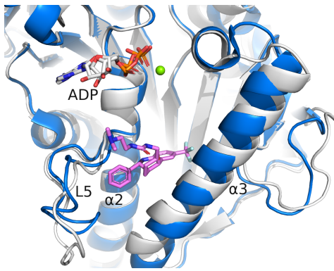
EMD 534085
