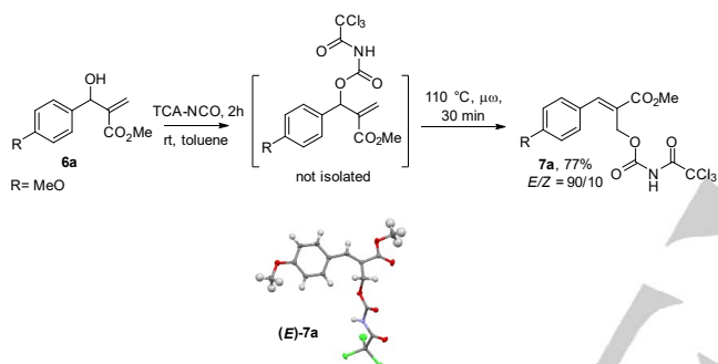
Scheme 2. Stereoselective synthesis of ( E )- 7a involving a microwave-assisted rearrangement.
