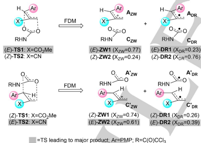
Scheme 5. Decomposition of saddle points TS1 and TS2 in the carboxylate (C) and allylic (A) fragments, according to the Fragment Distortion Model (see text). The contributions of the zwitterionic (ZW) and diradical (DR) resonance forms are also highlighted.
