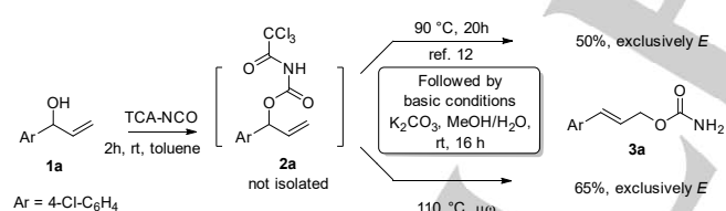
Scheme 1. Improvement of the tandem reaction using the microwave heating.
