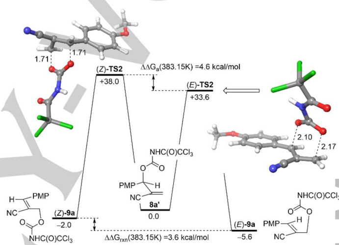
Figure 3. Reaction profile of the dioxo-[3,3] sigmatropic shift of carbamoyl intermediate 8a' to both ( E ) and ( Z ) isomers of 9a . See Figure 2 caption for additional details.
