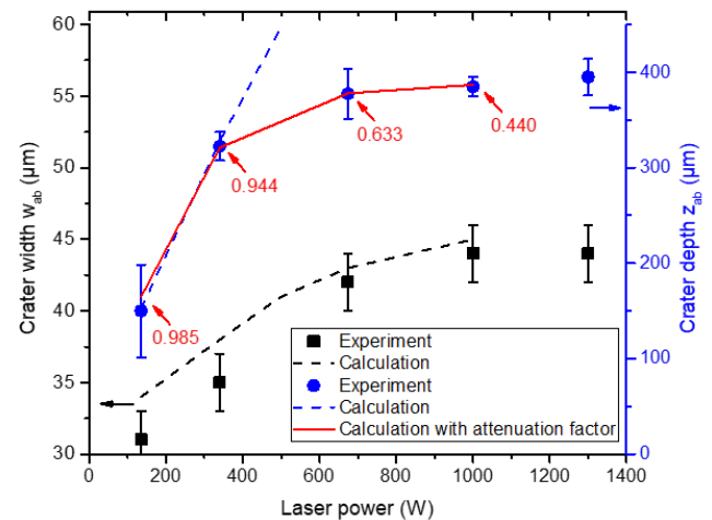
Fig. 4. Experimental crater depth z_{ab} (blue dots) and diameter w_{ab} (black dots) as a function of laser power. The black and blue dashed lines are the corresponding numerical results. The red line indicates the depths obtained with the model considering the attenuation factors (the numerical values are indicated for each power).
