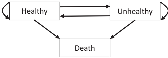
Fig. 2. Depiction of possible transitions among health states.
