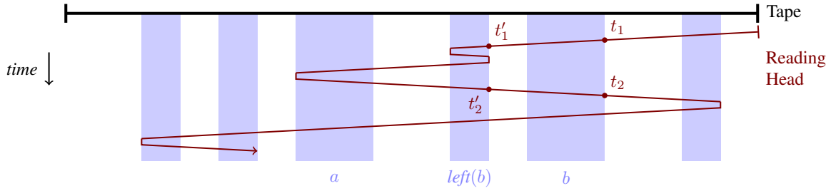
Figure 11: Illustration of t'_1 and t'_2 when b is skipped. The detour on \text{left}(b) is not required but clarifies the definition of t'_2 .
