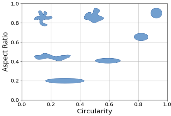
Fig. 4: Expected NP shapes according to the values of circularity and aspect ratio.
