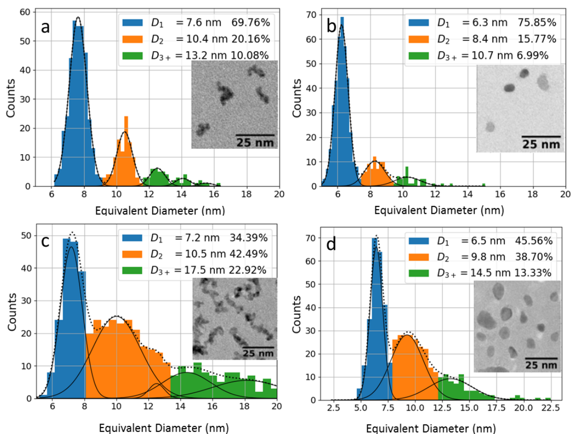
Fig. 1: Size histograms with N-Gaussian fit (black curves), separation of NPs population in monomers D_1 (in blue), dimers D_2 (in orange) and the rest as D_{3+} (in green) with corresponding % of NPS and TEM image in insert, for LD as prepared (a), LD annealed (b), HD as prepared (c) and HD annealed (d) large FeRh samples.
