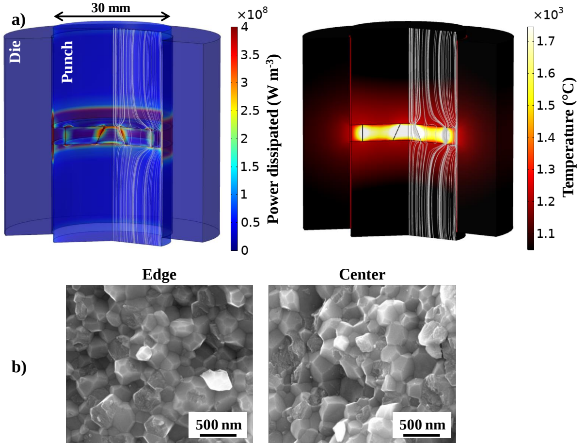
Fig. 4 Physical field uniformity and correlation with obtained microstructures. The upper part (a) shows the temperature distribution and electric current lines during the electric current peak, the lower part (b) represents the SEM fracture images in the center and at the edge of the sintered sample which demonstrate a homogeneous microstructure with grain size clearly lower than 500 nm.
