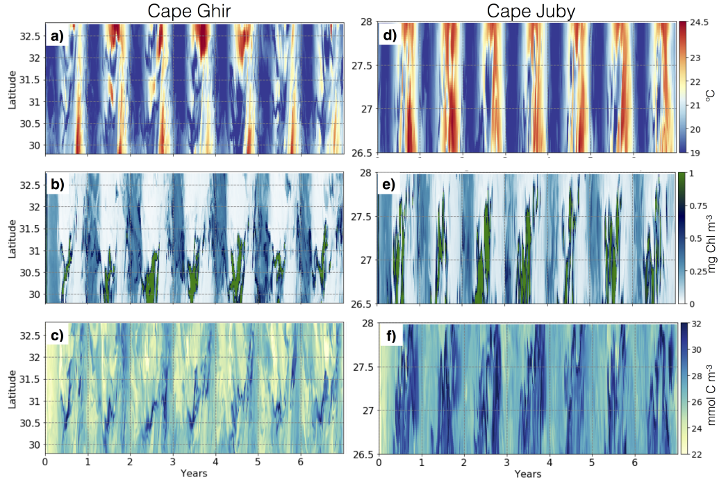
Figure 10: Latitude/time plots showing six repeated yearly cycles of 3-day averages of temperature ( ^{\circ} C; top panel), chl- a ( \text{mg Chl m}^{-3} ; middle panel), and e-TOC ( \text{mmol C m}^{-3} ; lower panel) off Cape Ghir (at 10.6^{\circ} W; left column) and Cape Juby (at 14.6^{\circ} W; right column), at 25 m depth.
