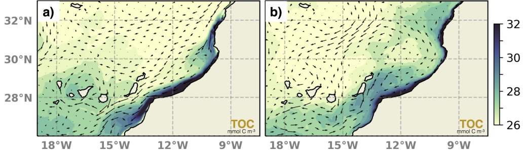
Figure 11: Plan view maps of e-TOC averaged over the top 25 m ( \text{mmol C m}^{-3} ) with averaged horizontal velocity vectors superimposed ( \text{m s}^{-1} ) for spring (a; left panel) and autumn (b; right panel) situations. Spring includes April, May, and June. Autumn includes October, November, and December.
