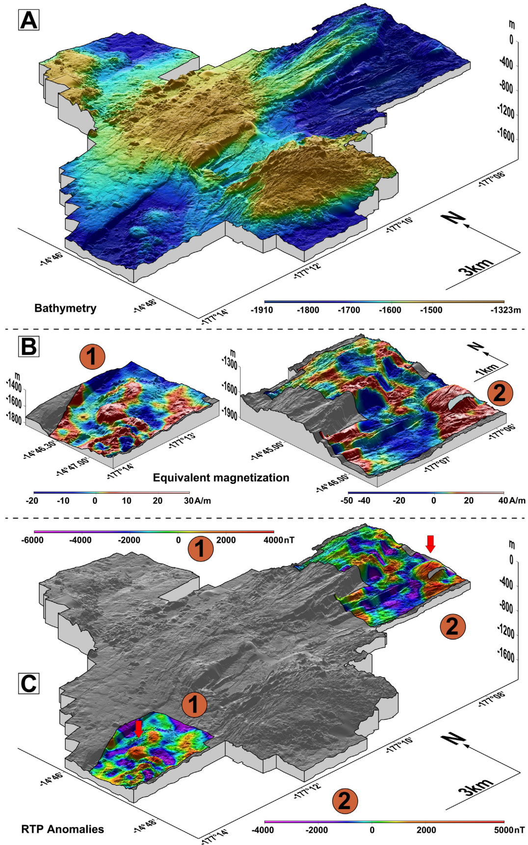
Fig. 4. (A) High-resolution bathymetry of the Fatu Kapa area. The central graben bisecting the area hosts the studied volcanoes in its eastern and western parts. (B) Equivalent magnetization derived from the AUV magnetic anomalies as in Fig. 2B for the studied volcanoes. (C) Reduced-to-the-Pole magnetic anomaly as Fig. 2C for the studied volcanoes. The volcanoes are associated with a positive equivalent magnetization and RTP magnetic anomalies consistent with a normal magnetic polarity.
