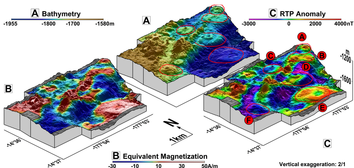
Fig. 5. (A) High-resolution bathymetry of the Tasi Tulo area. (B) Equivalent magnetization derived from the AUV magnetic anomalies as in Fig. 2B. (C) Reduced-to-the-Pole magnetic anomaly as Fig. 2C. Two volcanic ridges show a positive equivalent magnetization and RTP anomaly, whereas a series of at least six flat large volcanoes show variable magnetic signatures consistent with either normal or reverse magnetic polarities. B and E have a magnetic signature comparable to that of the Kulo Lasi whereas D and F are similar to Ono, with a rim of negative RTP magnetic anomaly encompassing an area of weaker magnetic signature.
