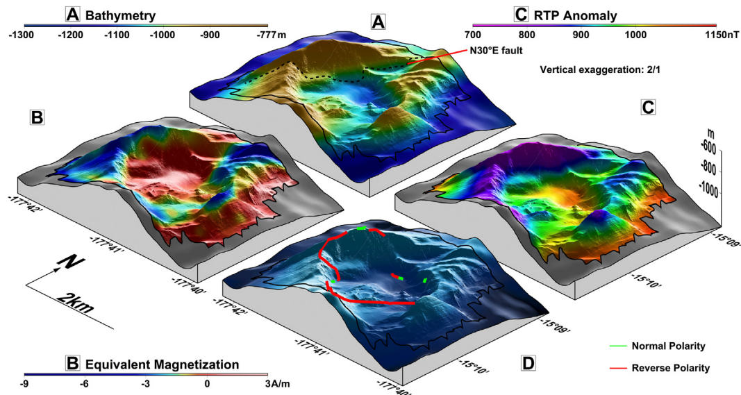
Fig. 3. (A) High-resolution bathymetry of the inactive Ono Caldera. Its bottom is smoothed by sediment coverage. (B) Equivalent magnetization derived from the AUV magnetic anomalies as in Fig. 2B. (C) Reduced-to-the-Pole magnetic anomaly as in Fig. 2C. The RTP anomaly is opposed to that of the Kulo Lasi Caldera (Fig. 2C) and requires a reversed magnetic polarity. (D) Magnetization intensity and polarity along the DSS Nautila path. The polarity is consistently reversed, confirming the result from the AUV data.
