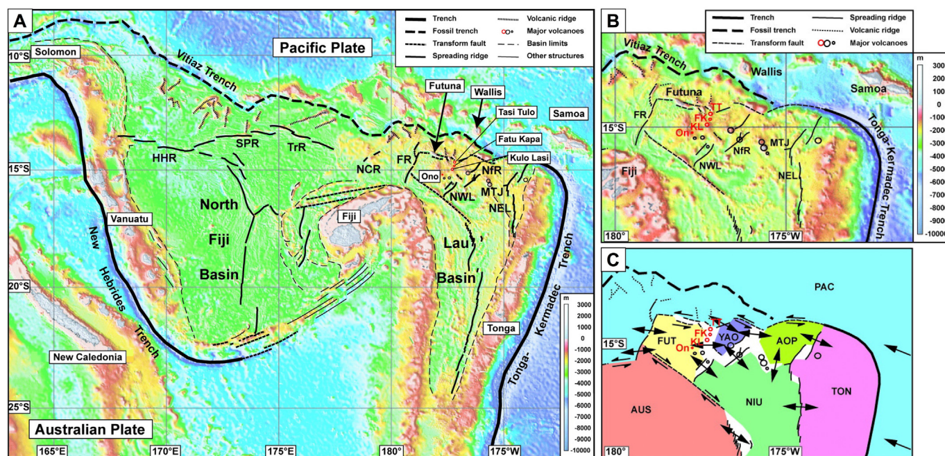
Fig. 6. (A) See Fig. 1A. (B) Regional bathymetry and tectonic structures in the northern Lau Basin. Abbreviations: see Fig. 1A and KL, Kulo Lasi; On, Ono; FK, Fatu Kapa; and TT, Tasi Tulo. (C) Plates and their inferred relative motions in the northern Lau Basin (modified after Zellmer and Taylor, 2001 and Bird, 2003). Plain colors describe individual plates: AUS, Australian Plate; PAC, Pacific Plate; TON, Tonga Plate; NIU, Niuafo'ou Plate; FUT, Futuna Plate; AOP, An Other Plate; YAO: Yet Another One. The three later plates are proposed in this study. Double-headed arrows: diverging motion; Double arrows: transform motion; Single-headed arrows: converging motion.
