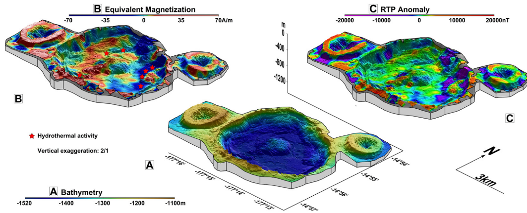
Fig. 2. (A) High-resolution bathymetry of the Kulo Lasi Caldera. The smooth bathymetry at its bottom corresponds to new and mostly basaltic lava flows with some andesitic flows. (B) Equivalent magnetization derived from the AUV magnetic anomalies using Honsho's Bayesian inversion (2012). (C) Reduced-to-the-Pole magnetic anomaly computed from the equivalent magnetization. The bottom of the caldera is associated with a relatively weak magnetic anomaly by comparison with the top of the two flanking volcanoes. To the Northeast, an elongated negative magnetic anomaly corresponds to a hydrothermally active area, in accordance with previous studies in basaltic (e.g., Tivey et al., 1993) and andesitic (Fujii et al., 2015) contexts.
