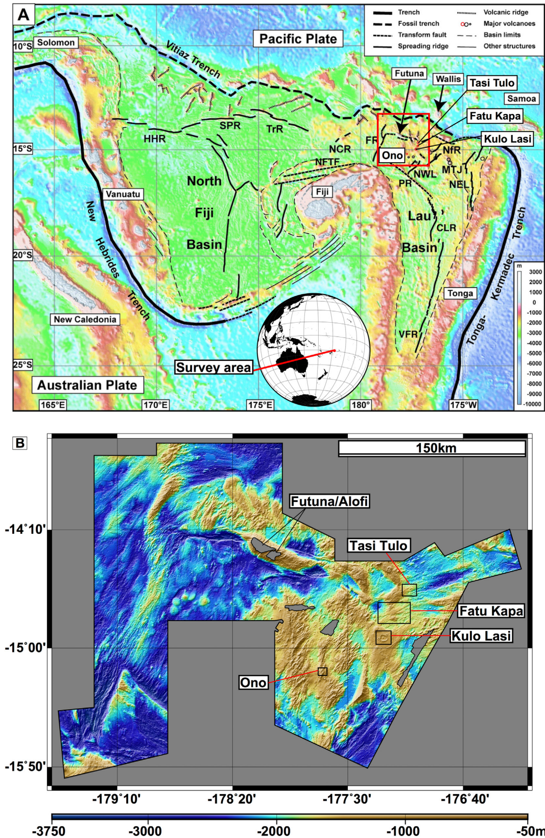
Fig. 1. (A) Regional bathymetry and tectonic structures of the North Fiji and Lau basins. Bathymetric background from Ruellan and Lagabrielle (2005). HHR, Hazel-Holmes Ridge; SPR, South Pandora Ridge; TrR, Tripartite Ridge; NCR, North Cikopia Ridge; FR, Futuna Ridge; NWL, Northwest Lau Ridge; NEL, Northeast Lau Ridge; NRR, Niufo'ou Ridge; MTJ, Mangatolu Triple Junction; NFTF, North Fiji Transform Fault; PR, Peggy Ridge Transform Fault; CLR, Central Lau Spreading Center; VFR, Valu Fa Spreading Center. Many large volcanic ridges and edifices lie in a 200 km-wide stripe south of the fossil Vitiaz subduction zone. (B) Close-up on the Futuna area based on the bathymetric data from cruises ALAUI and FUTUNA 1, 2 and 3, with Futuna and Alofi Islands in the center of the map. The bathymetry to the Southeast of the islands is generally shallower than to the West, marking the SEFVZ. The Kulo Lasi Caldera, Fatu Kapa and Tasi Tulo areas are located within the dashed rectangle whereas the inactive Ono Caldera is located slightly further to the Southwest.
