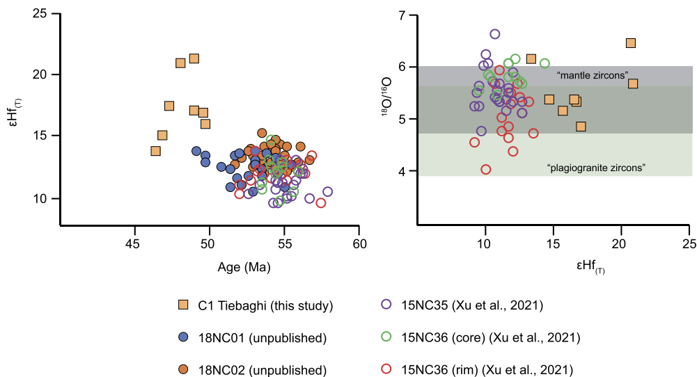
Fig. 4. Plots of \epsilon\text{Hf}(t) vs. age and VSMOW-normalised \delta^{18}\text{O} vs. \epsilon\text{Hf}(t) for the youngest, potentially magmatic zircon population in the C1 Tiébaghi sample allowing comparison with zircons from Eocene dykes that intrude the Peridotite Nappe elsewhere. Zircons from samples 15NC35 and 15NC36 were collected near Népoui in the Kopeto massif (Xu et al., 2021) and samples 18NC01 and 18NC02 are unpublished data of J.C.A., D.C. and R.J.Z. from Eocene-age zircons in dykes from near Coulée in the massif du Sud.
