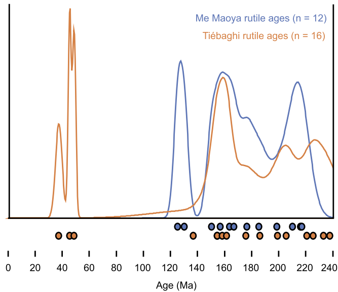
Fig. 7. Histogram of U-Pb ages obtained for rutiles collected from the Tiébaghite chromitite and Me Maoya harzburgite.
