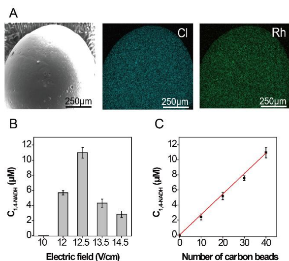
Figure 2. (A) SEM image of a CB-Rh bipolar electrode and the corresponding elemental mapping. Scale bar is 250 μm. Bipolar electrochemically produced NADH concentration (B) as a function of the applied electric field with 40 carbon beads and (C) as a function of the number of CB-Rh beads at an electric field of 12.5V/cm. Experiments were carried out with cell 1 (see supporting information for details), CB-Rh electrodes in 10mL PBS pH 7.0 in the presence of 5 mM ascorbic acid and 1 mM NAD +
