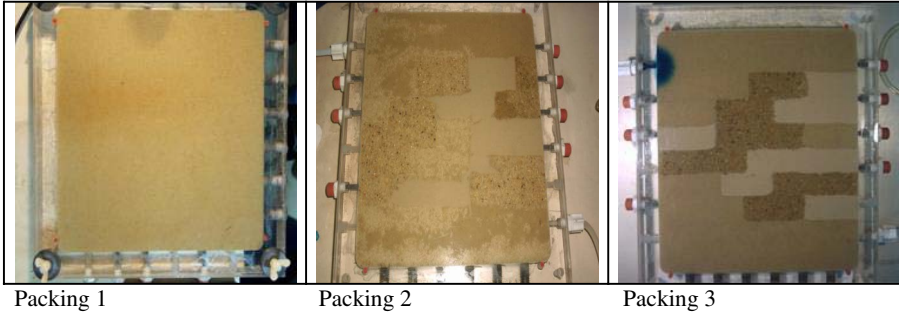
Fig. 1. Sand packing arrangements used for the laboratory experiments. Packing 1: homogeneous packing with medium sand. Packing 2: heterogeneous packing arrangement with coarse, medium and fine sand. Packing 3: heterogeneous packing arrangement with coarse, medium and fine sand.
