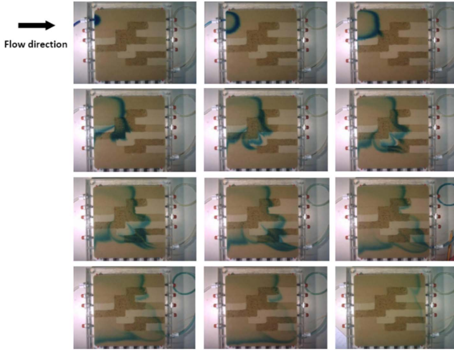
Fig. 4. Spatial evolution over time of tracer (blue dye) injected into Packing 3. Photographs are taken at approximately uniform time intervals over approximately one hour. (For interpretation of the references to color in this figure legend, the reader is referred to the web version of this article.)
