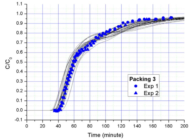
Fig. 15. Comparison between measured BTC and BTCs from 30 Monte Carlo simulations (Packing 3).
