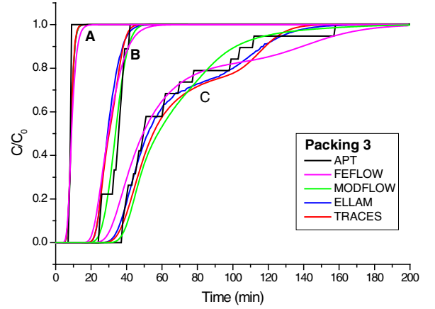
Fig. 12. Simulated breakthrough curves for Packing 3 at points located in A (8.1, 17.3), B (11.3, 7.3) and C (17.6, 14.9); see Fig. 3.
