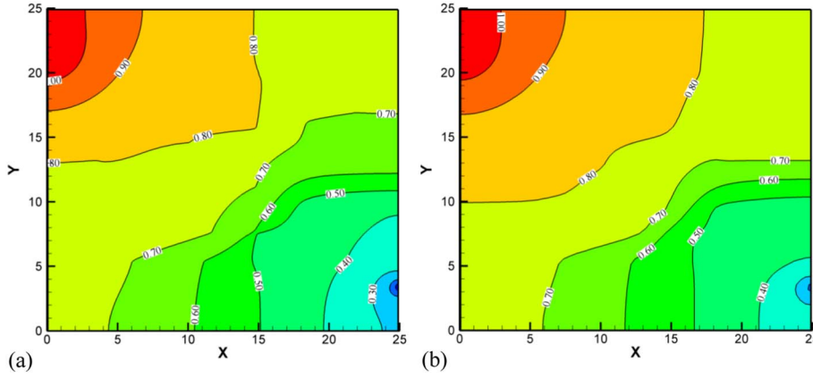
Fig. 7. Pressure head distribution for Packing 2 and spatial discretization of (a) \Delta x = 1 mm and (b) \Delta x = 4 mm.
