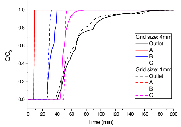
Fig. 6. Simulated breakthrough curves for Packing 3 considering advective transport only at points located in A (8.1, 17.3), B (11.3, 7.3) and C (17.6, 14.9); see Fig. 3.
