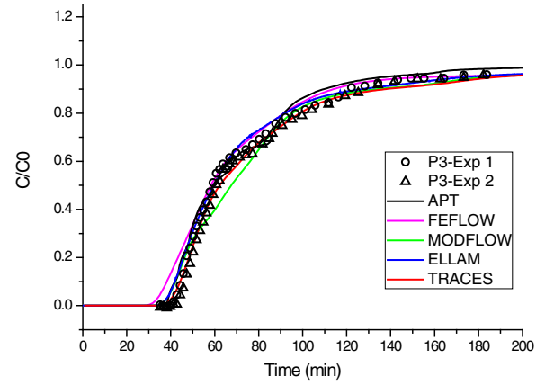
Fig. 10. Measured and simulated breakthrough curves at outlet for Packing 3 (P3).
