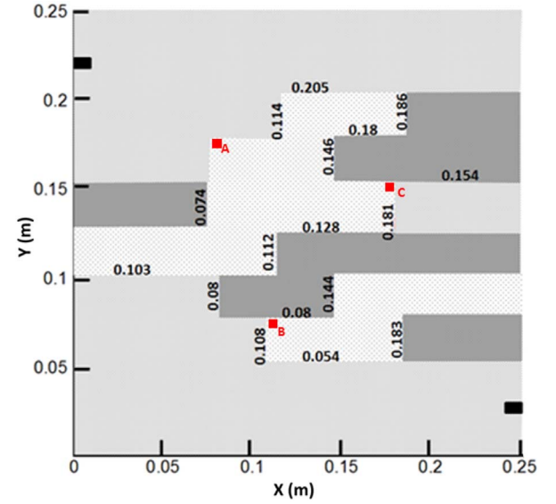
Fig. 3. Disposition of coarse (light grey), medium (grey) and fine (dark grey) sands in the Packing 3. Decimal values within the domains denote the coordinates in meters of each boundary ( x and y dimensions are written vertically and horizontally, respectively). Inlet and outlet in each domain are represented by the black rectangles at the upper left and lower right sides, respectively. Red squares represent the locations where internal BTCs are computed. (For interpretation of the references to color in this figure legend, the reader is referred to the web version of this article.)
