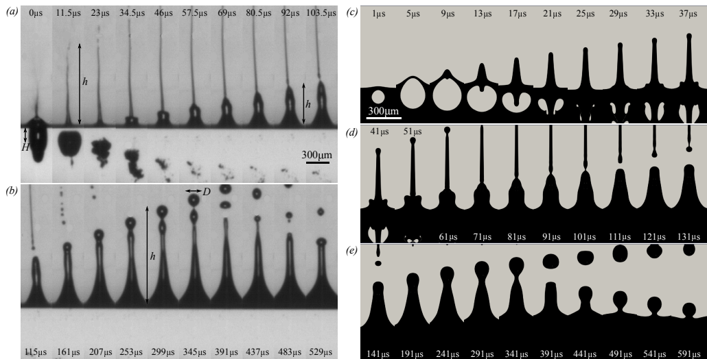
FIGURE 1. (a)-(b) Sequence of side-view images illustrating the experimental bubble and jet dynamics, the nucleation depth H , the jet height h and the droplet diameter D . The laser pulse energy is E = 18.3 \mu\text{J} and H = 144 \mu\text{m} . The first thin jet appears concomitantly with the bubble expansion while the second jet emerges \sim 30 \mu\text{s} later when the bubble has deflated and recoiled away from the interface. (c)-(e) Numerical analog of the experimental images. Vertical slices ( y-z plane) of the 3D numerical simulations of the bubble and jet dynamics. Here H = 80 \mu\text{m} and the initial bubble pressure is P = 600 bars. The second jet is beginning to emerge \sim 30 \mu\text{s} after initiation. The simulations reproduce the main features of the experiments and show additional details such as the counter-jet ( t = 17 \mu\text{s} ) not easily observed in our experiments.
