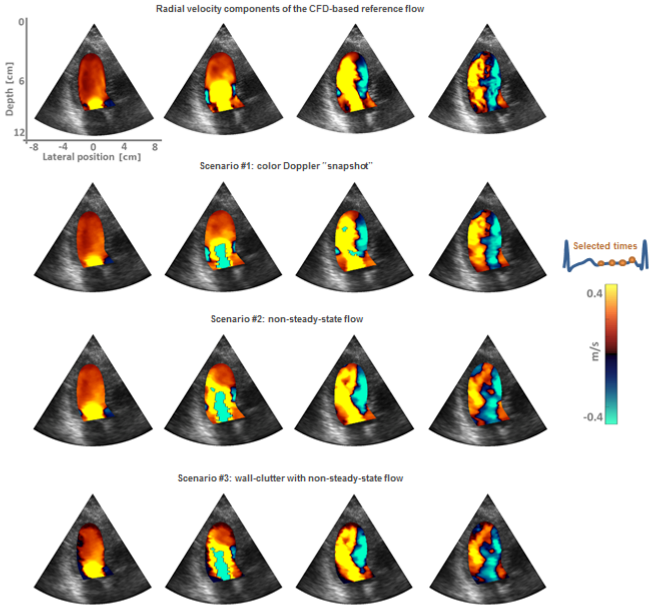
Fig. 6: Illustration of the ability of our Doppler simulation pipeline to generate three different types of scenarios: 1) a color Doppler “snapshot” situation assuming a stationary flow and the absence of myocardial motion (second row); 2) unsteady flow where the blood scatterers are relocated between two successive ultrasound transmits (third row); 3) wall-clutter with unsteady flow where both the blood and tissue scatterers are relocated between two successive ultrasound transmits (fourth row).
