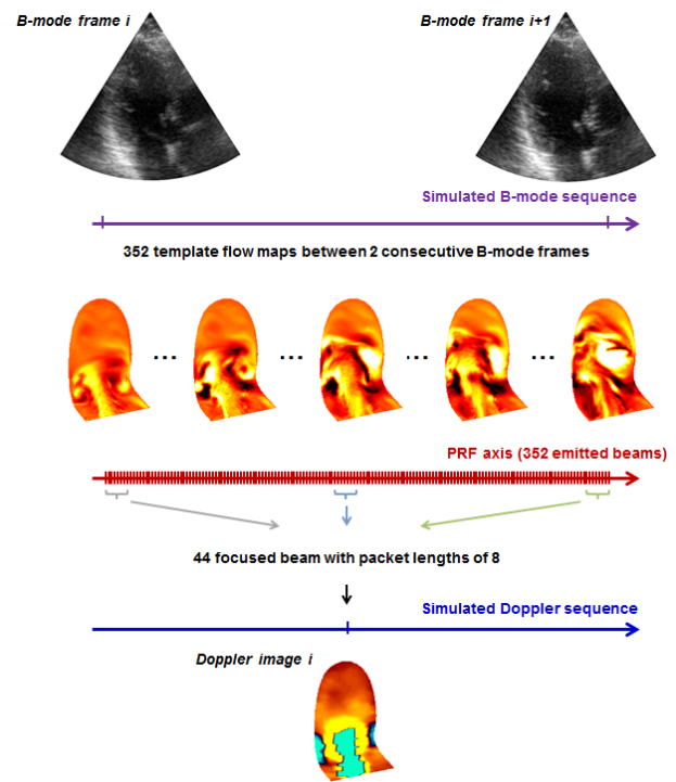
Fig. 5: Overall strategy for the simulation of Doppler images. 352 registered flow maps were used between each consecutive B-mode frame. This leads to a different map per emitted beam at the PRF frequency. 44 focused beams with a packet length of 8 were used to estimate each color Doppler image.
