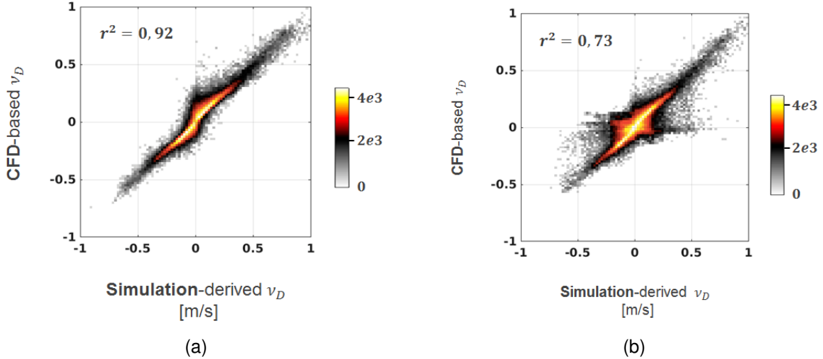
Fig. 9: CFD-based vs, simulation-derived Doppler velocities ( v_D ) for (a) the scenario #1 and (b) the scenario #1 with additional wall clutter noise. Velocity data from sixteen Doppler images for five different virtual patients.
