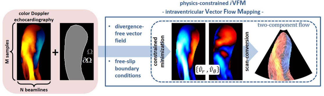
Figure 2. The physics-constrained iVFM algorithm is written as a minimization problem constrained by two physical properties: mass conservation and no penetration boundary conditions. It works with color Doppler velocities before scan conversion, in a polar coordinate system (leftmost images). \Omega represents the domain of interest (left ventricular cavity), and \partial\Omega is its boundary (endocardial wall). Reproduced from Assi et al (2017). © 2017 Institute of Physics and Engineering in Medicine. All rights reserved.
