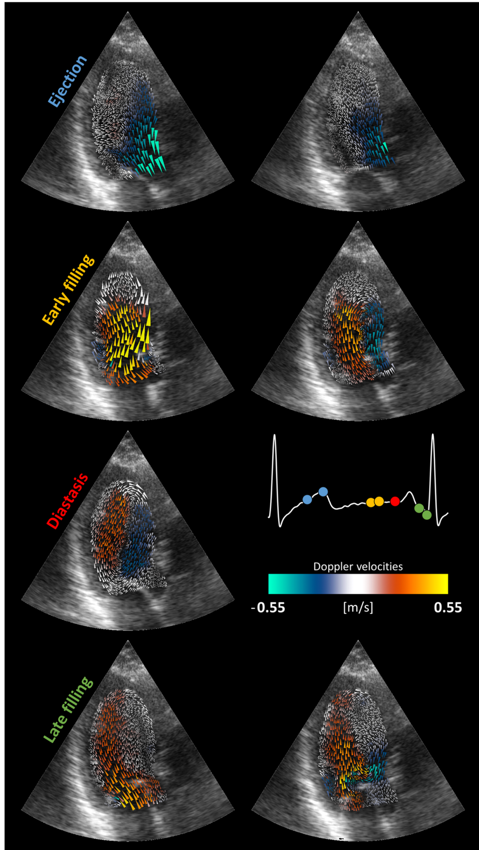
Figure 11. Physics-constrained intraventricular vector flow mapping (iVFM) in a patient. Selected frames show blood inflow and outflow in the left ventricle. The large vortex that forms during early filling is visible during diastasis. The color of the arrows represents the original color Doppler fields from which the iVFM fields were deduced.
