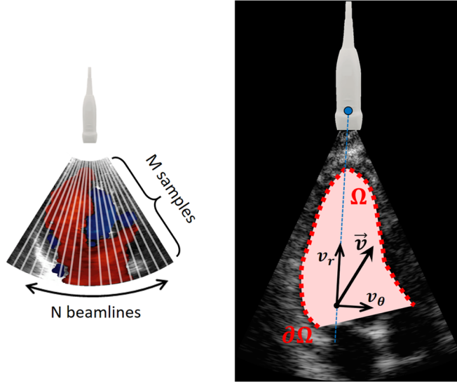
Figure 1. The physics-constrained iVFM algorithm is implemented in the polar coordinate system associated with the color-Doppler sector. Physics-constrained iVFM returns a 2D velocity field \vec{v}(r, \theta) from the Doppler components by minimizing a cost function subject to constraint equalities. \Omega represents the domain of interest, and \partial\Omega is its boundary.
