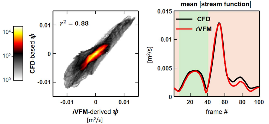
Figure 10. Left: CFD-based versus iVFM -derived stream function. Data from the 100 CFD images were pooled. The binned scatterplot (left panel) displays the number of velocity occurrences. Right: Spatial average of the absolute value of the stream function.
