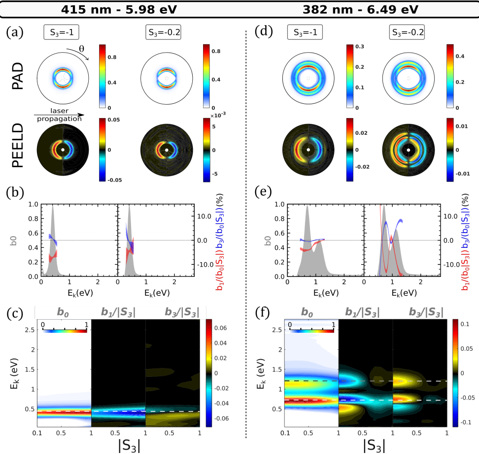
Fig. 6 2D PAD and PEELD recorded in (2+1) REMPI at 415 nm (a-c) and 382 nm (d-f). (a,d) Abel-inverted PAD and PEELD images recorded with S_3 = -1 and S_3 = -0.2 . The PAD is normalized to its own maximum and the PEELD to the PAD maximum. (b,e) Kinetic energy distributions of the Legendre coefficients b_0 (in grey), b_1/|S_3| (in red) and b_3/|S_3| (blue) for these two ellipticities. The b_{1,3}(E)/|S_3| coefficients are normalized to b_0(E, |S_3|) . (c,f) b_i/|S_3| parameters as a function of |S_3| and the kinetic energy. Both b_{1,3}(E, S_3)/|S_3| are normalized to the maximum value of b_0(E, |S_3|) . b_0(E, S_3) is normalized to its own maximum over all the S_3 recording. In the (c,f) panels, the horizontal lines indicate the kinetic energies expected from E_k = \hbar\omega_0 - IP_a + E_R for 3s and 3p bands using the E_R binding energies listed in Table 1. The white dashed line is for 3s and the white-gray one for the 3p band.
