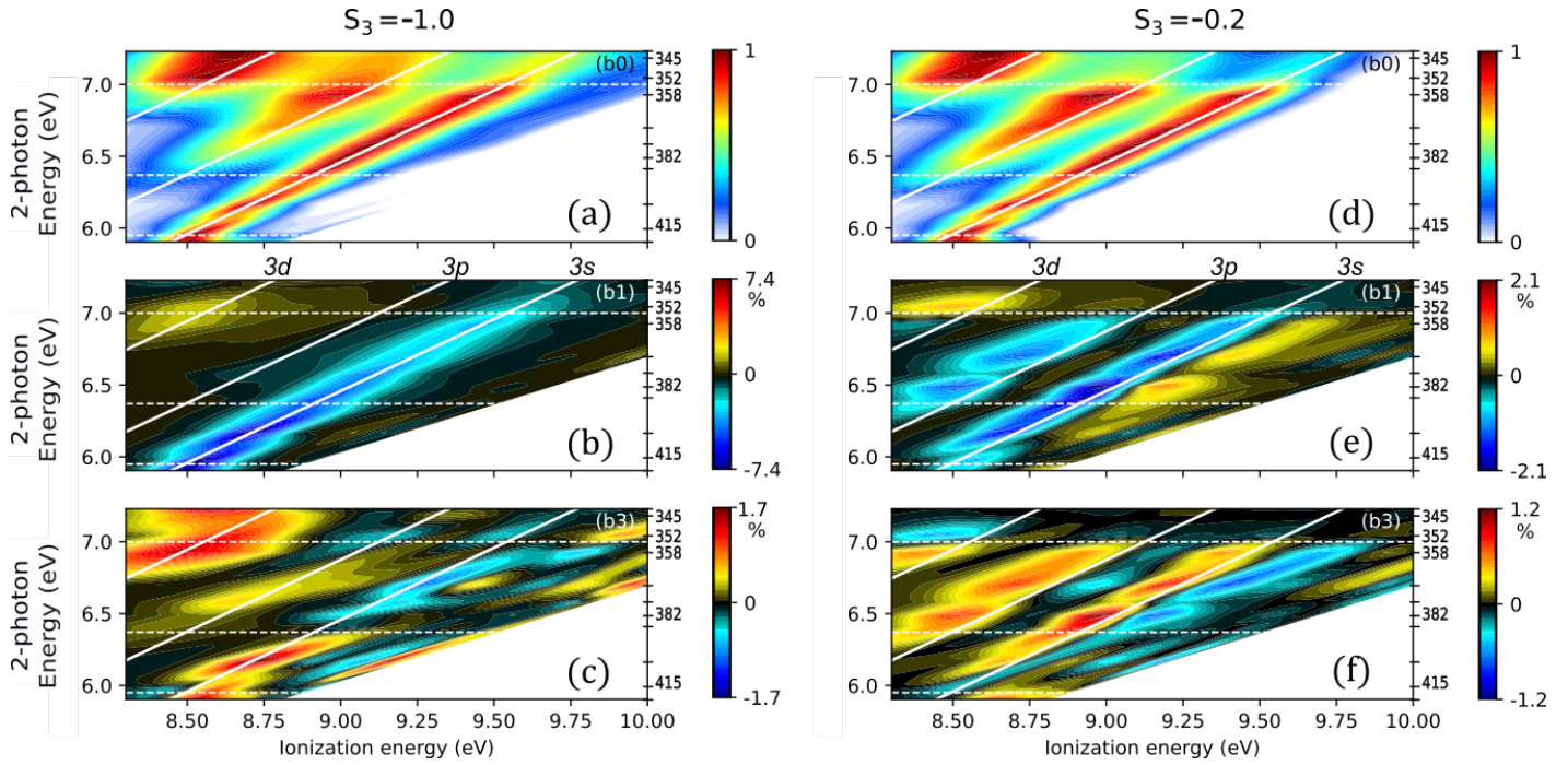
Fig. 4 Legendre decomposition of the REMPI photoelectron signal as a function of the two-photon excitation energy and the ionization energy ( IE = 3 \times \hbar\omega_0 - E_k = I_{pa} - E_R + 2\hbar\omega_0 ), for (a-c) a circular polarization S_3 = -1 and (d-f) elliptical polarization ( S_3 = -0.2 ) with (a,d) refers to b_0 , while (b,e) correspond to b_1 , and (c,f) to b_3 . The 11 excitation wavelengths used in this study are indicated on the right side of each graph and the five ones leading to remarkable transitions in the ionization dynamics are mentioned in nm. For each excitation wavelength, the coefficients are normalized to the maximum of b_0 . The 3s, 3p and 3d Rydberg series are identified by the continuous diagonal white lines corresponding to the \Delta\nu=0 propensity rules of ionization with binding energies E_R = 5.95 eV, 6.37 eV and 6.94 eV respectively (see Table 1). The horizontal dashed lines indicate the thresholds of appearance of 3s, 3p and 3d bands on the PEELD maps. Note that the Legendre decomposition of (2+1)-REMPI PAD also involves a b_5 coefficient which has been found negligible in all cases.
