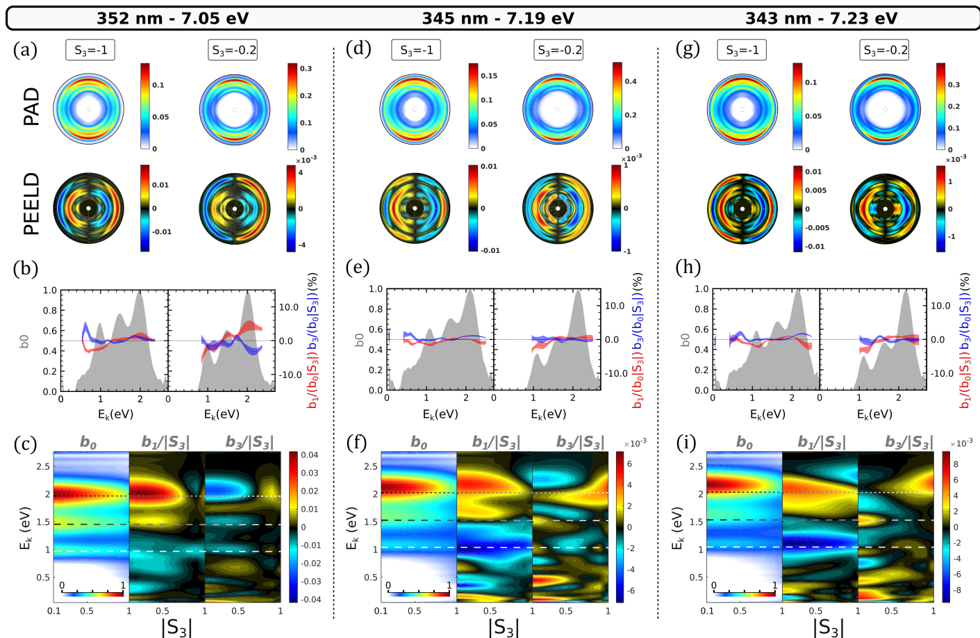
Fig. 9 Same as Figure 6 for two-photon excitation energies within the 3d band.
