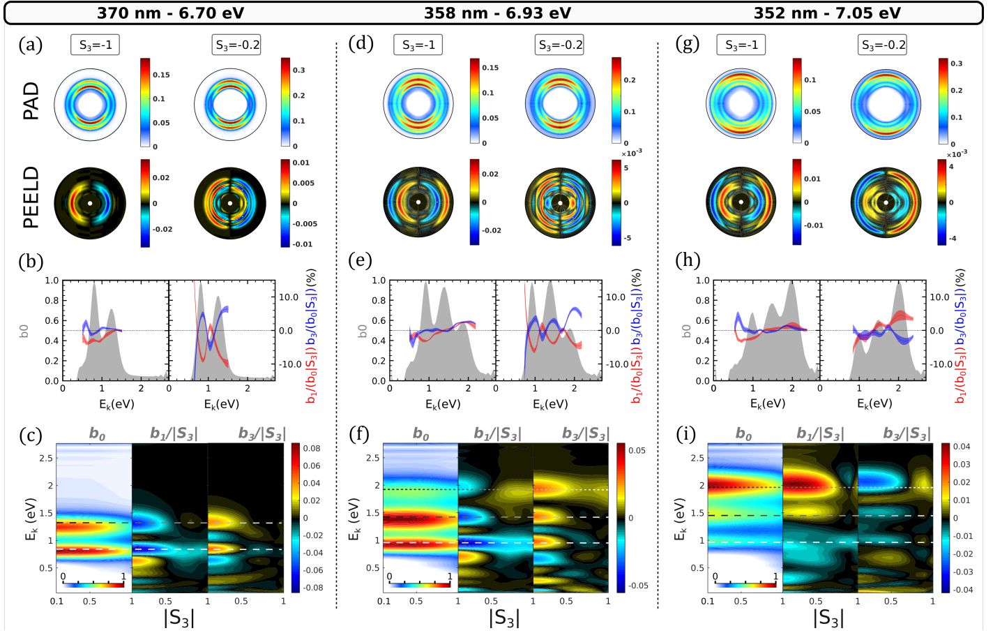
Fig. 7 Same as Figure 6 but for two-photon excitation energies reaching the 3d band. In the (c,f,i) panels, the horizontal lines indicate the kinetic energy expected from E_k = \hbar\omega - IP_a + E_R for 3s, 3p and 3d bands using the E_R binding energies listed in Table 1. The white dashed line is for 3s state, the white-gray one for the 3p band and the dot white-gray line for the 3d band.
