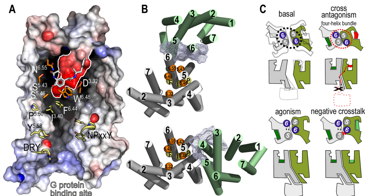
Fig. 5. Mechanisms of type I allostery in GPCR oligomers heteromers. (A) Cross-section through a prototypical class A GPCR, highlighting the agonist (white sticks), the amino acids of the orthosteric site (delineated by a white line) involved in ligand binding (orange), the conserved PIF motif (yellow), and the NPxxY and DRY motifs and Y, (yellow) that transmit the signal from the PIF motif (transmission switch) to the G protein site (Weis & Kobilka, 2018). (B) Position of these amino acids involved in ligand binding (orange spheres) and signal transmission (yellow) in models of GPCR dimers via TM5 and TM6 (top) and TM4 and TM5 and intracellular loop 2 (bottom). Clearly, a ligand-bound (type I allostery) or ligand-free (type II allostery) or orphan GPCR (green cylinders) can modify the affinity (orange spheres) or efficacy (yellow spheres) of the partner receptor (gray) via the protein-protein interface (blue mesh). (C) GPCRs are dynamic proteins that adopt, in a ligand-free form, a number of conformations (shades in gray) that not only involve the extracellular and intracellular sites (Weis & Kobilka, 2018), but also a potential TM oligomeric interface. An inverse agonist (red polygon) binding to one of the protomers of a GPCR heteromer triggers a high surface complementarity between TM5 and TM6 of the two molecularly different protomers, via the four-helix bundle (dashed red circle) (Manglik et al., 2012), which blocks the opening of the intracellular cavity for G protein binding at the other protomer (cross-antagonism) (Viñals et al., 2015). An agonist (green polygon) binding to one of the protomers triggers the outward movement of TM 6 (see arrows), opening the intracellular cavity for G protein binding (Rasmussen et al., 2011), whereas the TM5 and TM6 heteromeric interface impedes simultaneous agonist-induced movement of both TM6 (negative crosstalk) due to a steric clash (red cross) (Guinart et al., 2020).
