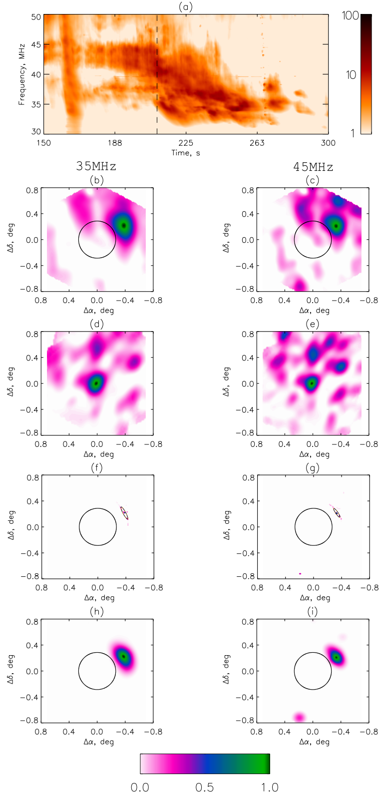
Figure 6. Solar radio map deconvolution procedure. Panel (a) shows the dynamic spectrum, the logarithm of intensity vs. time and frequency, for the considered event (a transitioning type II burst, reported by Chrysaphi et al. (2020)), with the X-axis showing time in seconds after 10:59:38 UT on 2017 July 15. Panels (b) and (c) show dirty maps observed at 11:03:07 UT (shown as the black dashed line in panel (a)). Panels (d) and (e) show corresponding LOFAR PSFs derived using the combined PSF for the location of the Sun at the moment of observations. Panels (f) and (g) show corresponding clean component maps (color scales, Section 3.1) and their 2D Gaussian fits (black and orange dashed lines show their half-maximum contours, Section 3.2). Panels (h) and (i) show corresponding cleaned maps (as described in Section 3.1). Panels (b), (d), (f), and (h) are for 35 MHz; panels (c), (e), (g), and (i) are for 45 MHz.
