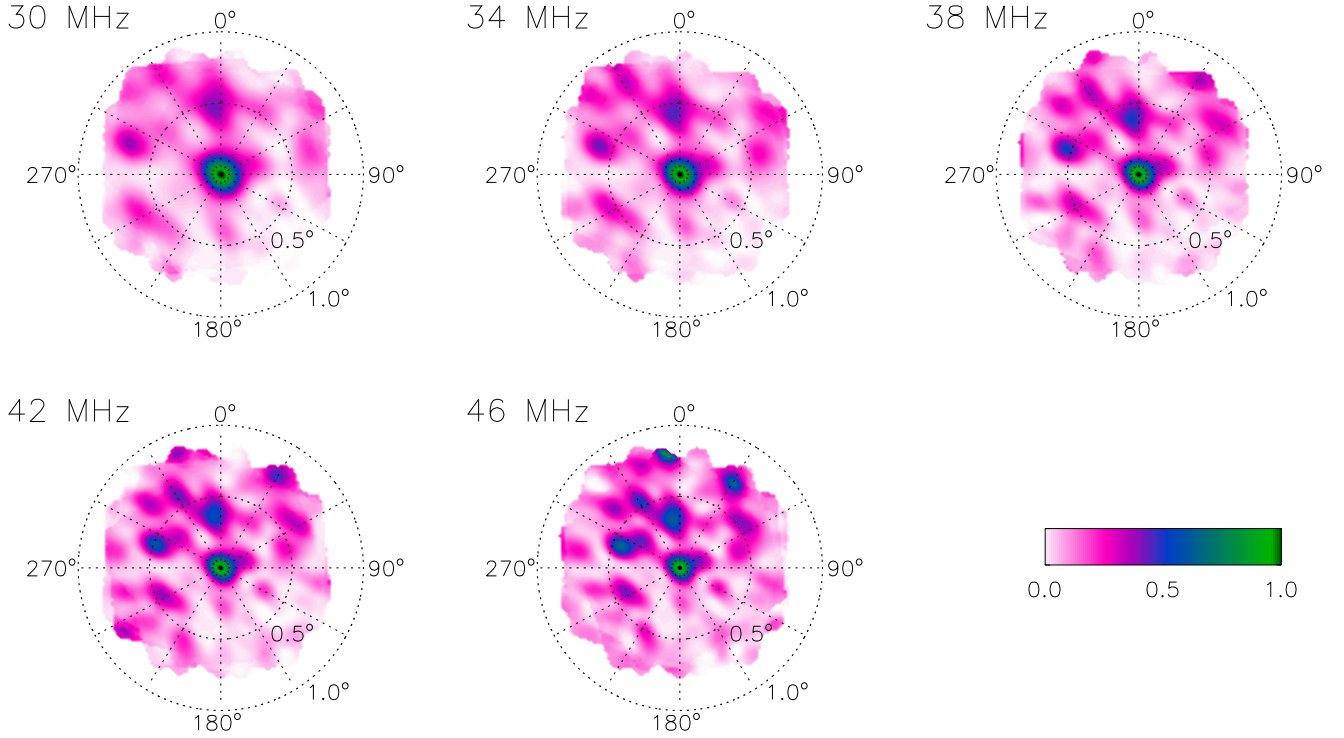
Figure 3. LOFAR PSF based on 22 Tau A observations projected to zenith above the LOFAR core. Frequencies are shown above the panels.
