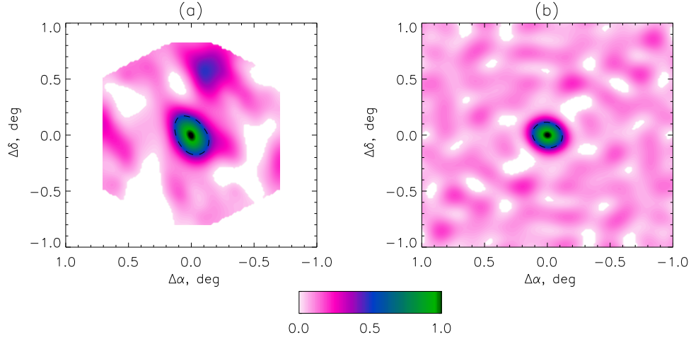
Figure 4. Tau A observed by LOFAR at 30MHz at 07:00 UT on 2017 July 13 compared with the nominal PSF of LOFAR calculated for the same frequency, time and sky coordinates.
