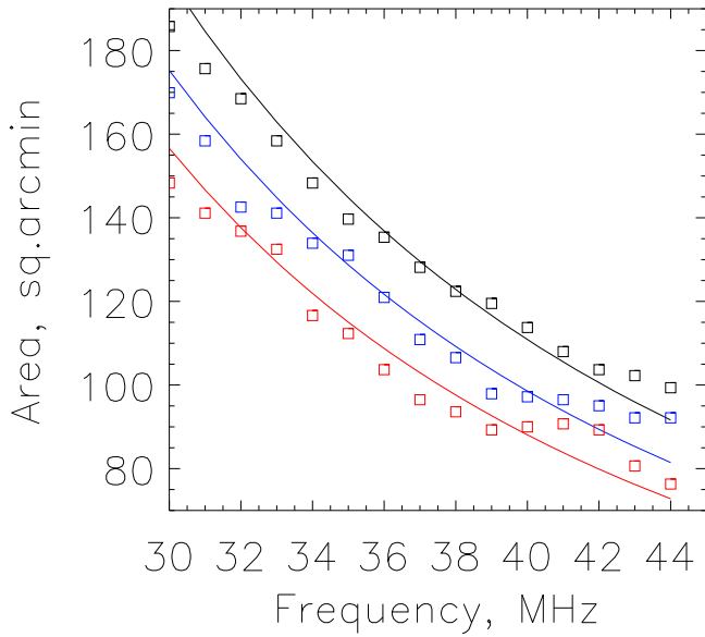
Figure 9. Area of the effective LOFAR PSF at zenith evaluated using different estimates for the constant background intensity. Black squares are for the PSF calculated with N=2 , blue and red squares are for N=109 and N=200 , respectively. Lines with corresponding colors show 1/f^2 data fits.
