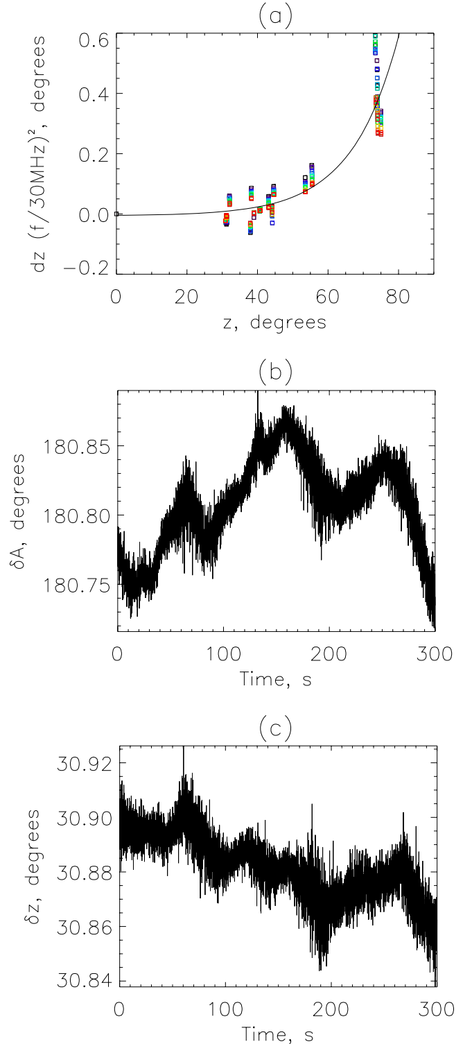
Figure 5. Panel (a) zenith distance offsets of Tau A centroids observed at different zenith distances. The values are normalized by f^2 factor to remove the effect of frequency variation (see Section 2.3). Different colors represent different frequencies from 30 MHz (black) to 48 MHz (red). The black line shows the analytical approximation for the \mathcal{R}(z) function. Panels (b) and (c) apparent azimuth and zenith distance of Tau A observed at 30 MHz with the motion due to the Earth rotation removed. Horizontal axis shows the time after 11:01 UT on 2017 July 12.
