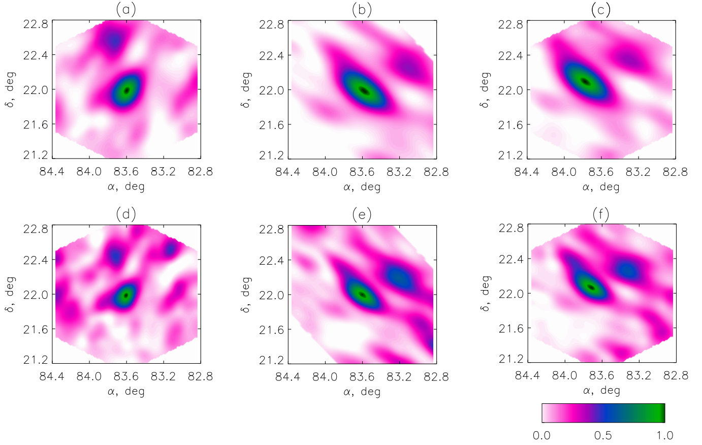
Figure 2. Left panels (a) and (d) show Tau A observed by LOFAR at 07:00 UT on 2017 July 13. Middle panels (b) and (e) show these intensity maps translated to the location where Tau A is observed at 10:05 UT on 2017 September 9. Right panels (c) and (f) show actual intensity maps of Tau A observed at 10:05 UT on 2017 September 9. Upper panels (a)–(c) correspond to the frequency 30 MHz, while lower panels correspond to 45 MHz.
