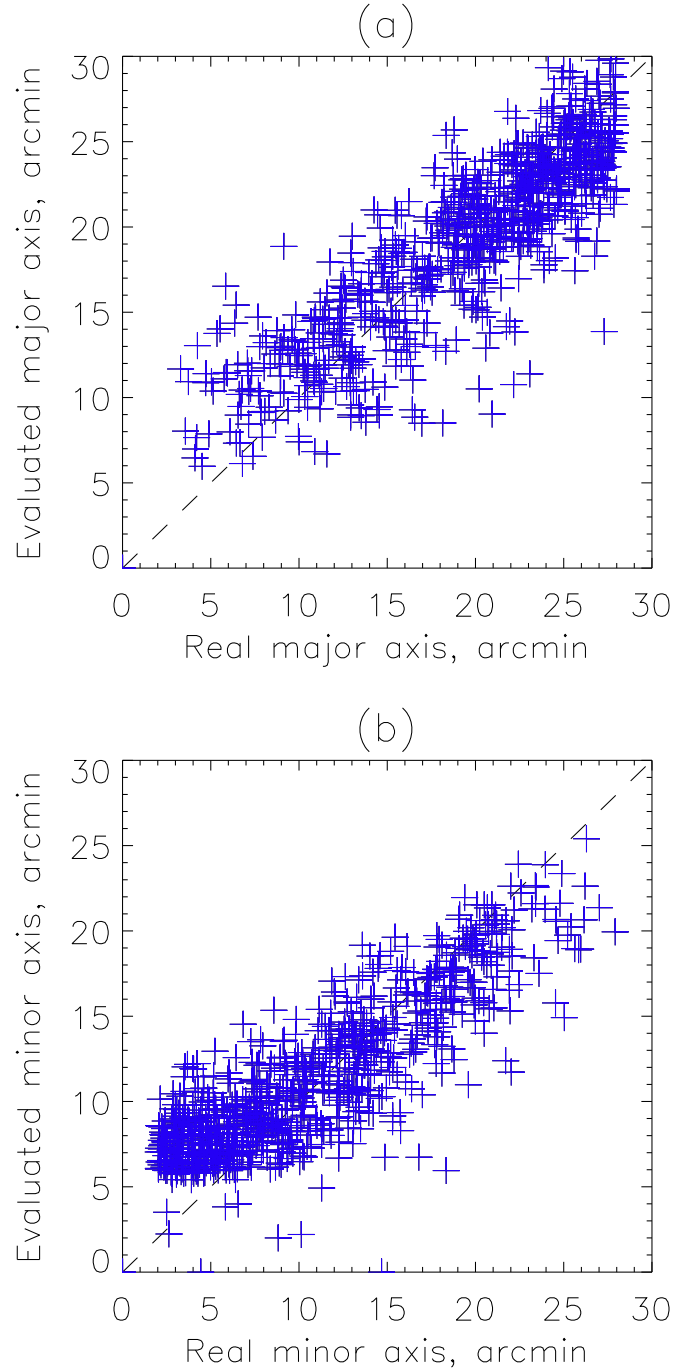
Figure 8. Comparison of the evaluated synthetic source sizes, major and minor axes of the half-maximum ellipses, with their actual values. The sizes were evaluated using the same set of procedures as used for solar data processing.
