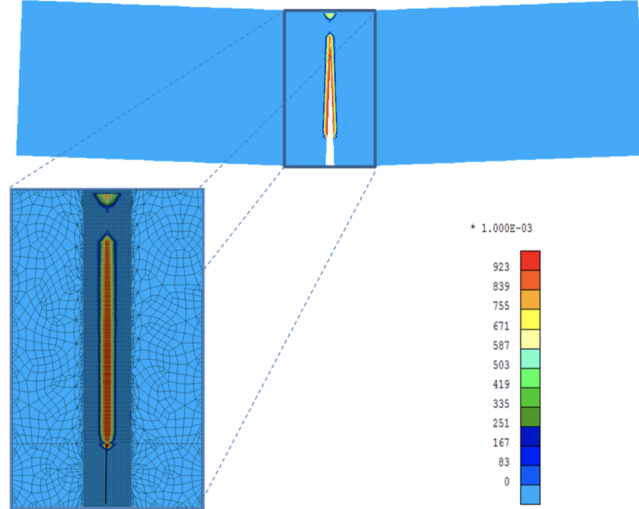
Figure 30: 3 points bending test: Damage distribution for NMOD=100 \mu m .
