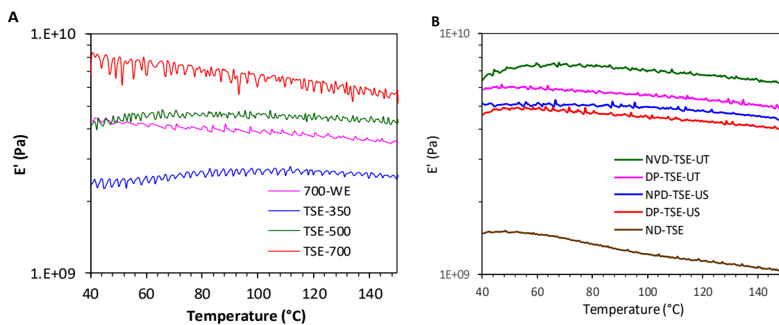
Figure S3. Storage modulus ( E' ) vs. temperature of thin film (A) from extruded fibers at different CCs during 30 min, and (B) from extruded fibers followed by UT or US treatment (TSE: 10 min at CC = 350 \mu\text{mol.g}^{-1} ; DP: dried pulp; NDP: never-dried pulp; UT: Ultra-Turrax during 5 min; US: ultrasonication during 1 min).
