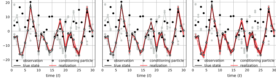
FIGURE 5. Comparison of CPF (left), CPFAS (middle), and CPFBS (right). The state (black line) and the observations (black points) have been simulated using the Kitagawa model (19) with Q = 1 and R = 10 . N_f = 10 particles (grey points with grey lines showing the genealogy) are used in the three algorithms. The red curves show N_s = 10 realizations simulated with the algorithms.
