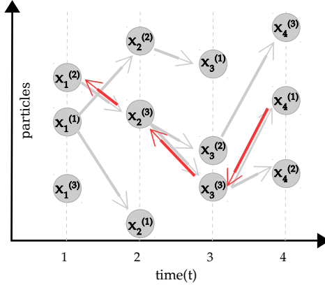
FIGURE 4. Example of ancestor tracking based on ancestral links of filtering particles. Particles (grey balls) are obtained using a filtering algorithm with N_f = 3 particles.
