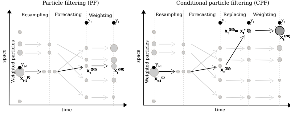
FIGURE 2. Comparison of one iteration of PF and CPF algorithms using N_f = 5 particles (light grey points). The differences are highlighted in black : CPF replaces the particle x_t^{(N_f)} of the PF with the conditioning particle x_t^* (dark grey point).
