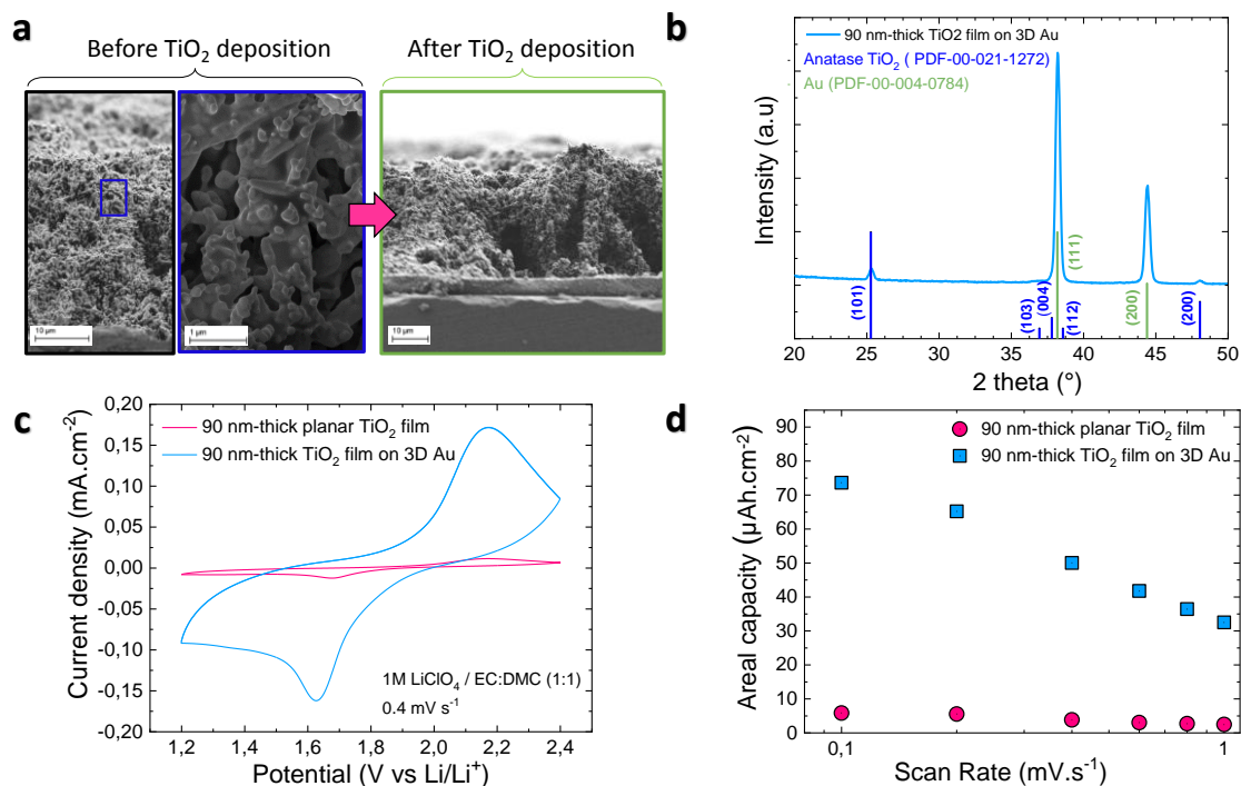
Fig. 1 | Preliminary studies on 3D porous gold metallic scaffold. a. Scanning Electron Microscope imaging of porous gold collector before and after the \text{TiO}_2 deposition by ALD at 200 ^\circ\text{C} . b. X-Ray Diffraction analysis of the 90 nm-thick \text{TiO}_2 film deposited on porous gold scaffold. c. CV profile of 90 nm-thick \text{TiO}_2 film deposited on planar Si wafer and 3D porous gold template. d. Evolution of the areal capacity vs the scan rate for 2D and 3D samples.
