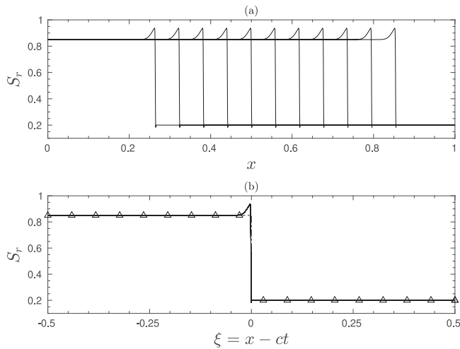
Fig. 5. One dimensional imbibition solution S_r of the coupled system Eq. (41), for \lambda = \rho_w g , S_r^0 = 0.20 and S_- = 0.85 ; (a) Solution at various time steps, (b) Solutions in (a) transformed into the TW-coordinate \xi = x - ct with c \approx 2.63 given by Eq. (34). Shock solution, Eq. (33), for S_- = 0.85 and S_+ = S_r^0 = 0.20 is shown with triangle markers.
