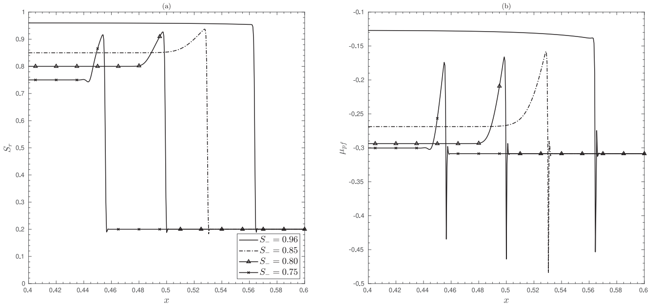
Fig. 4. One dimensional imbibition solutions of the coupled system Eq. (41), for \lambda = \rho_w g , with initial condition S_r^0 = 0.20 and boundary conditions corresponding to a constant rate of injection Eq. (43) with S_- = 0.96, 0.85, 0.80, 0.75 , \Delta t = 1\text{E-}05 , \Delta x = 5\text{E-}04 , (a) Saturation degree, S_r , (b) regularized effective chemical potential, \mu_{pf} . Solutions are shown at different time-steps and restricted spatial range for clarity. Out of this range, solutions are continuous and uniform extensions up to their respective boundary conditions.
