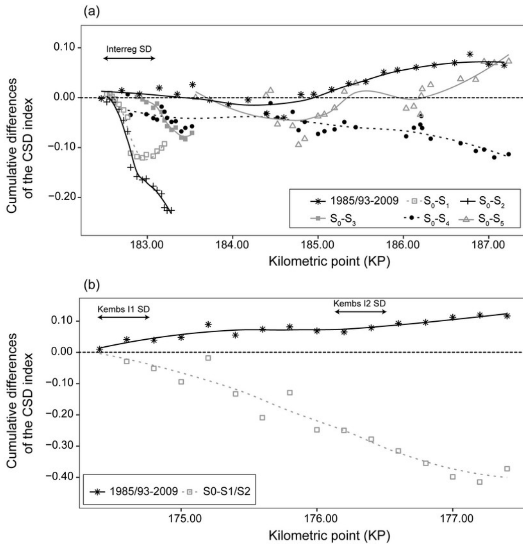
Figure 12: Cumulative differences in the CSD between the initial state and the successive surveys in the downstream direction (a) for the period 1985/93 - 2009 and S_0 to S_5 for the Interreg restored reach and (b) for the period 1985/93 - 2009 and S_0 to S_2 for Kembs I1 and S_0 to S_1 for Kembs I2.
