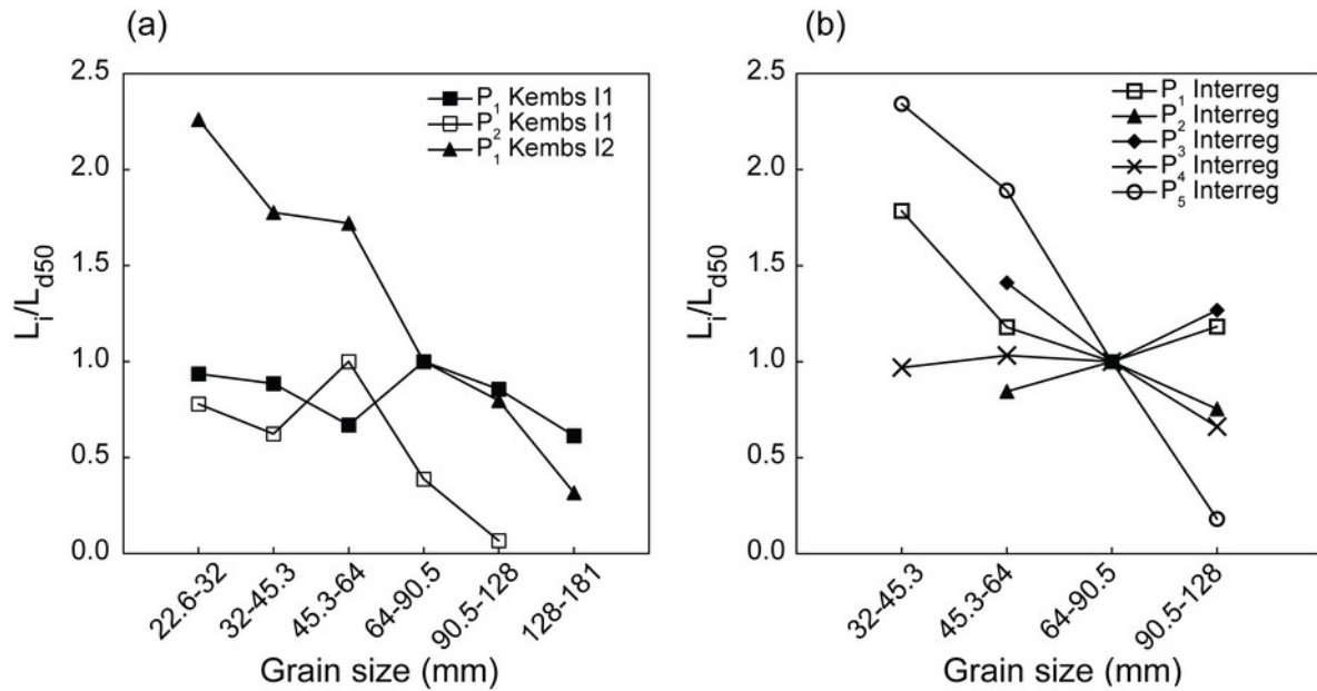
Figure 10: Mean dimensionless travel distance of the tracer cloud centroid for each grain size class, (a) for Kembs I1 and Kembs I2 and (b) for Interreg. Tracer clouds composed of less than 10 particles were excluded from the analysis because they were considered not statistically significant. For Kembs I1, only tracers recovered in the channel were included in the analysis.
