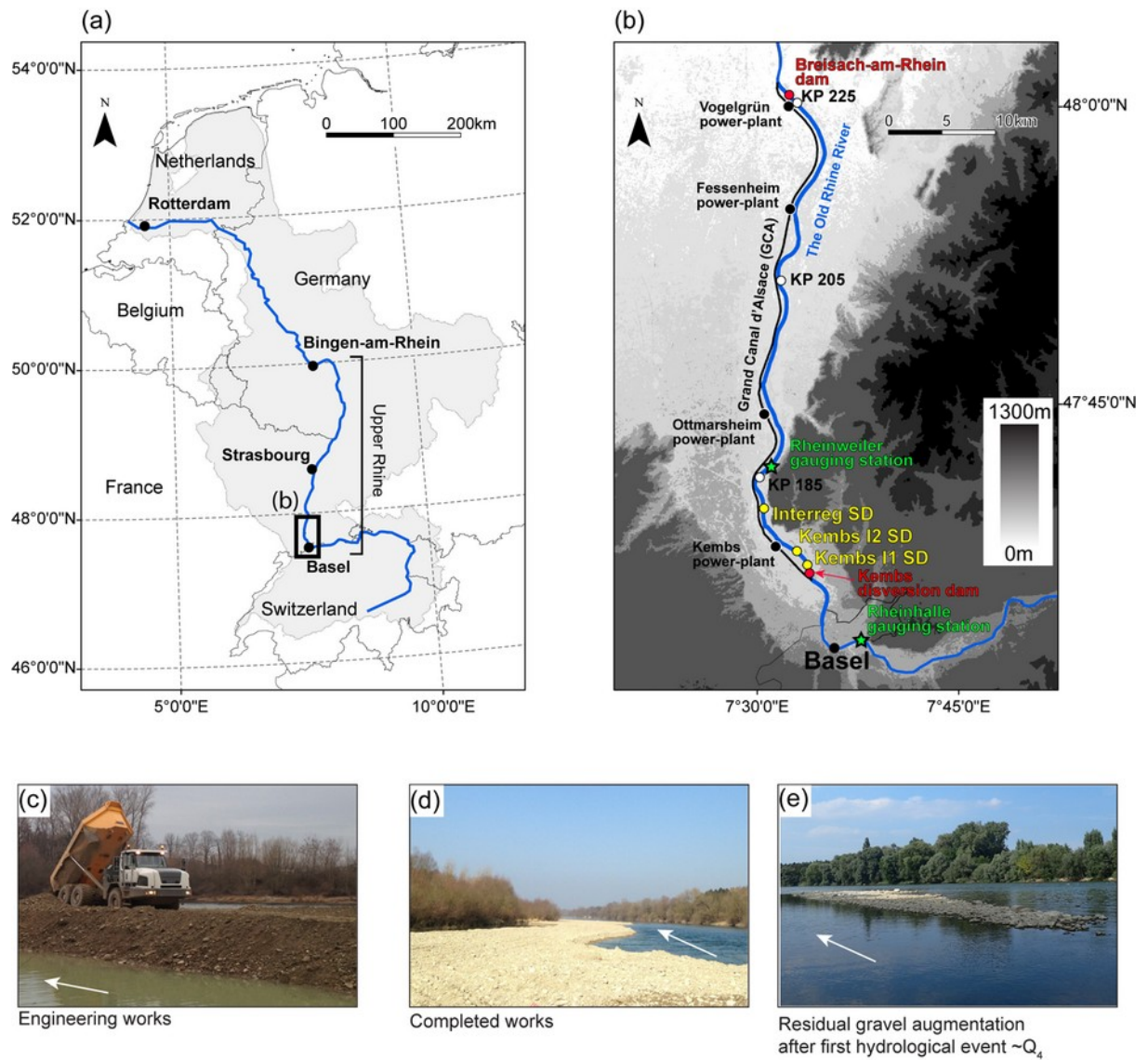
Figure 1: (a) Location of the Old Rhine river in the Rhine Basin, (b) location of the river network, the hydraulic structures, the gauging stations and the 3 GAs performed along the studied reach, (c) Kembs I2 SD in progress, (d) Kembs I2 SD completed and (e) residual Kembs I2 SD after a Q_4 flood in May 2016. White arrows indicate the flow direction.
