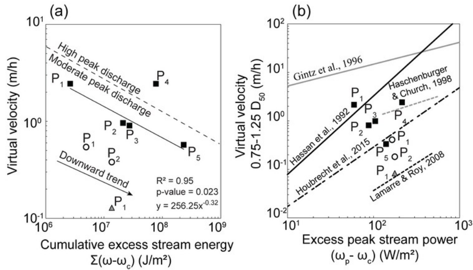
Figure 9: (a) Virtual velocity of the tracer cloud centroids for each P_i according to the cumulative excess stream energy and (b) virtual velocity of the tracer cloud centroids composed of tracers whose grain size ranges between 0.75 and 1.25 of the channel bed D_{50} as a function of the excess unit stream power for each P_i (modified after Houbrechts et al., 2015). The class 22.6-32 mm of Kembs I1 and Kembs I2 was excluded to make possible comparisons with Interreg. No relationship between the dimensionless travel distance of the tracer cloud centroid and the grain size classes of recovered tracers was found for Kembs I1 during P_1 , while a relation was observed during P_2 , indicating a partial mobility for this period (Figure 10). For Kembs I2, a marked negative relationship is observed between the two variables during P_1 , also indicating selective sediment transport. For Interreg, no relationship was found between the two variables up to P_4 . Thereafter, a marked negative relationship was established during P_5 , again showing selective transport.
