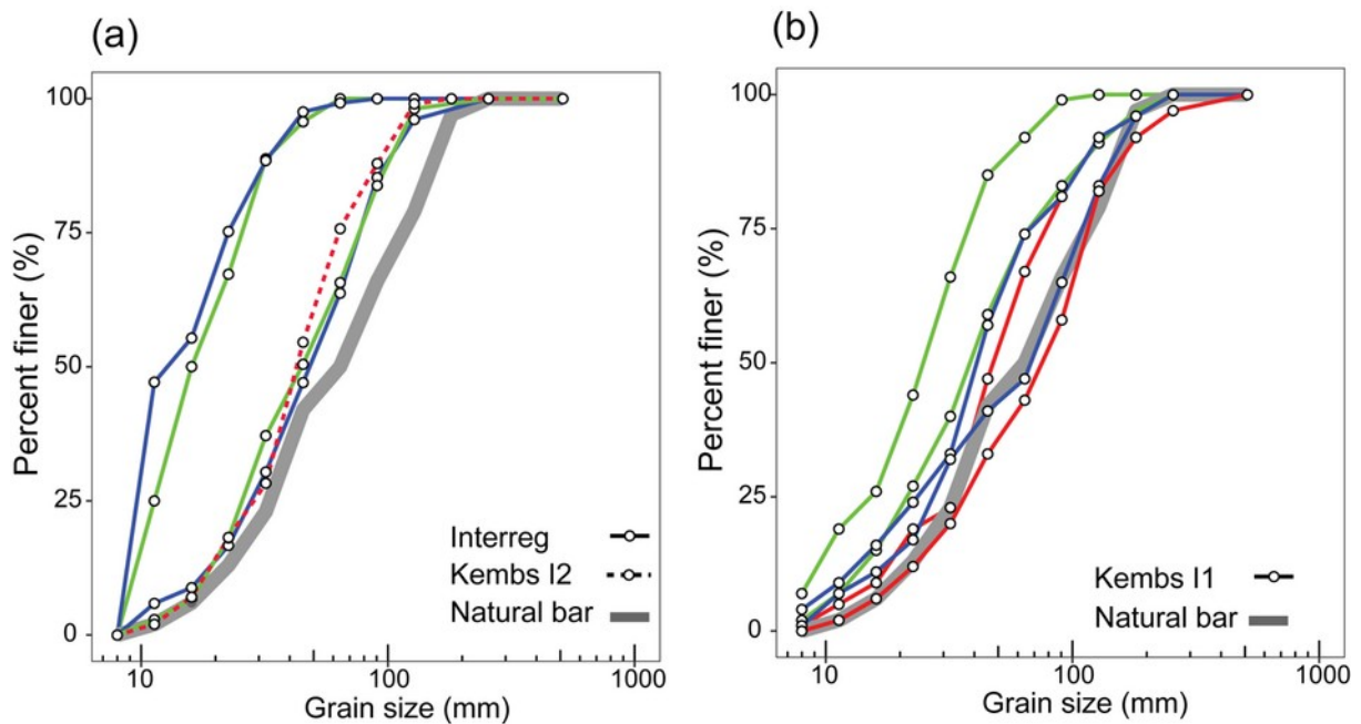
407 Figure 3: Surface grain size of the three residual SDs in S_1 (a) for Interreg ( n=4 ) and Kembs I2 408 ( n=1 ), and (b) for Kembs I1 ( n=6 ). Gray lines indicate the surface grain size of a gravel bar
