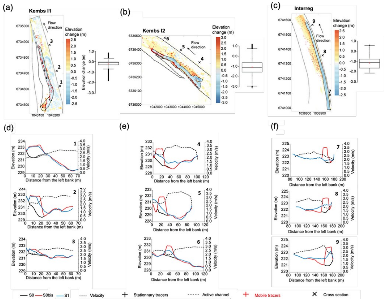
Figure 4: (a) to (c) DEM of differences from S_{Obis} to S_1 for the Kembs I1, Kembs I2 and Interreg SDs, with the location of mobile (red) and stationary tracers (black). Boxplots correspond to the elevation changes along each SD surface from S_{Obis} to S_1 . Intervals correspond to the 25 th and 75 th percentiles, and the lower and upper whiskers correspond to 1.5 times the interval quartile range. Black lines correspond to the median values, and the red points correspond to the mean values. (d) to (f) three cross sections extracted from DoD (cross symbol on (a) to (c)) illustrate the morphological changes for each SD from S_0 to S_1 .
