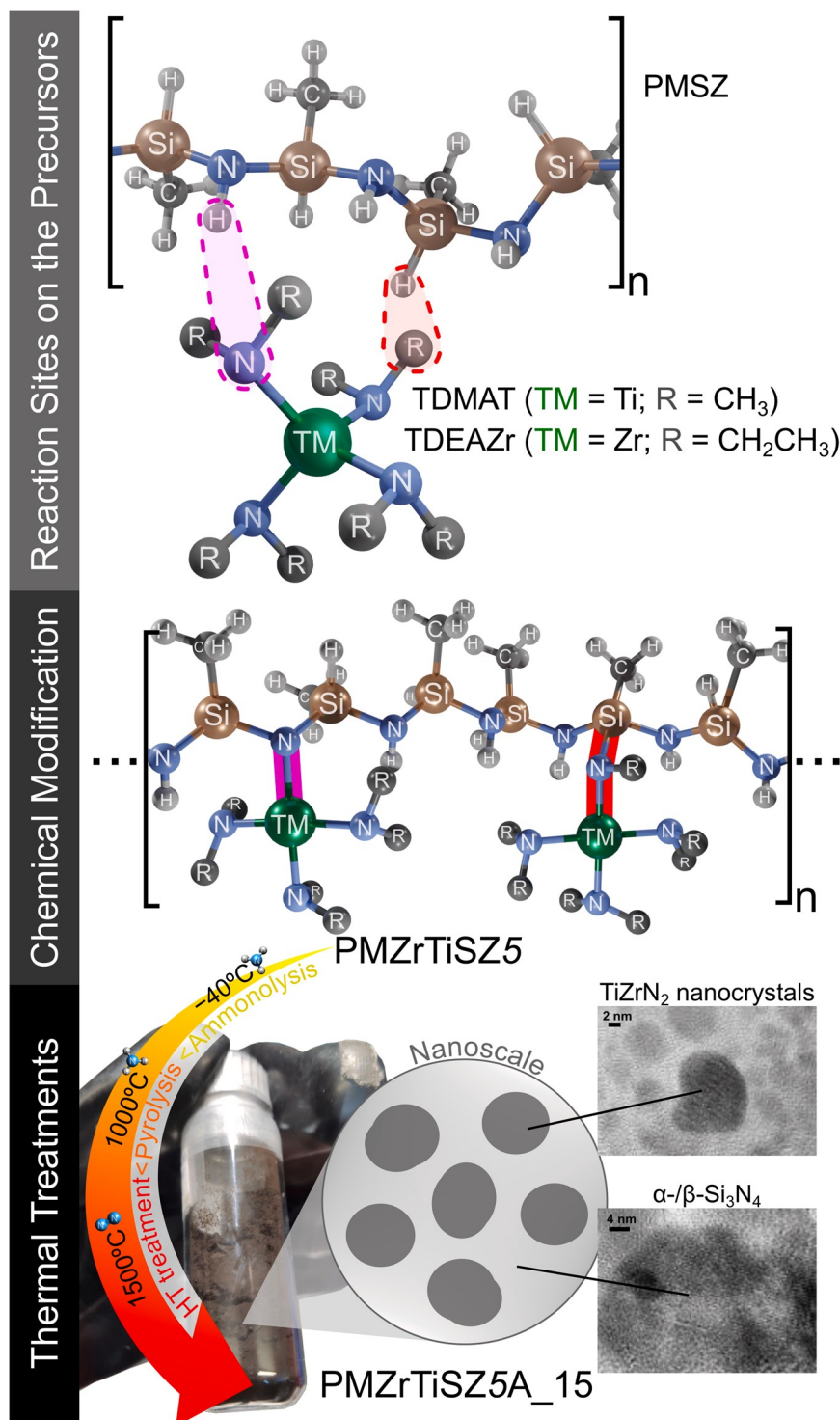
Fig. 1. Schematic diagram of the general process of designing TiZrN 2 /Si 3 N 4 nanocomposites from Ti and Zr-modified polysilazane.
