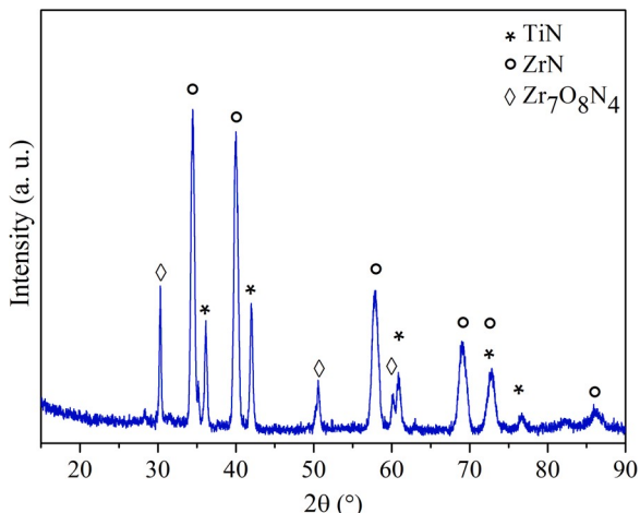
Fig. 6. X-ray pattern of TiNZrN_15 .
